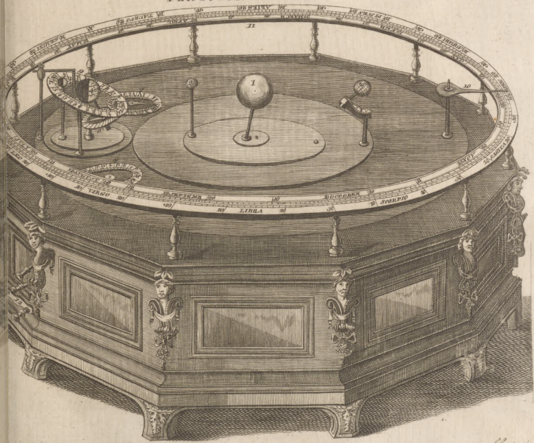
Fig. 3 FERGUSONS ORRERY
