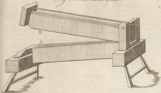
Fig. 1. Saw hand break
