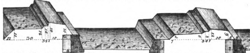
Profil of the Body of the Place and the Ravelin with demi-revetement
