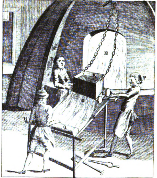
Fig. 2. Casting and Running of PLATE GLASS Plate XC VII
