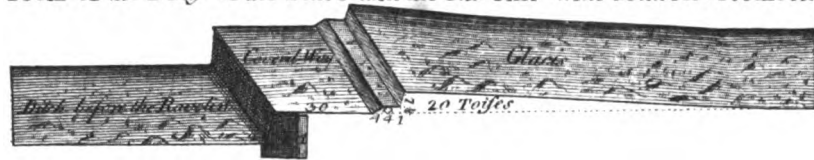
Profil of the Body of the Place and the Ravelin with demi-revetement
