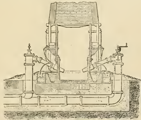
FIG. 30.—Refinery—Elevation.
