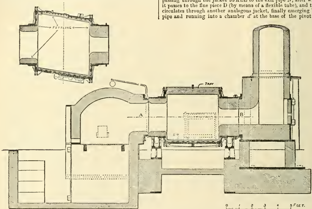
FIG. 38.—Spencer's Revolving Puddling Furnace. 1. Plan on line A B.
