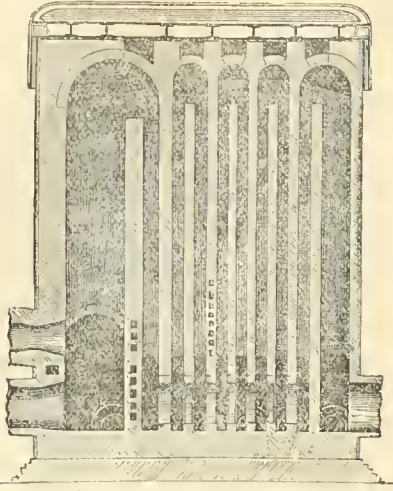
FIG. 19.—Whitwell Stove—Vertical Section.
