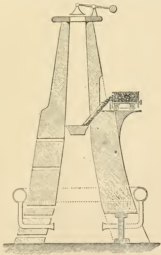
FIG. 2.—Westmann's Kiln.
