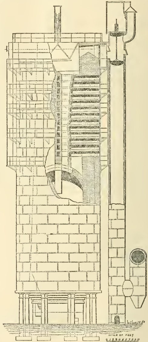
FIG. 13.—Ferrie's Furnace.
