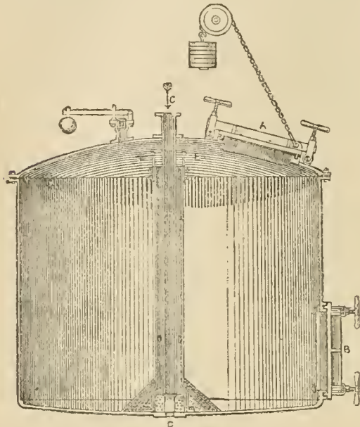
FIG. 1.—Section of Rag-Boiler.
