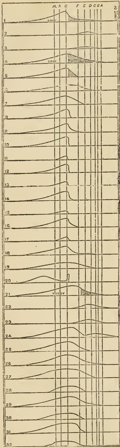
FIG. 1.—Spectrum Effects on Salts of Silver.
