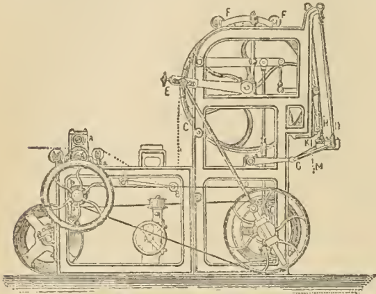
Fig. 9.—Single-Sheet Paper Cutter.
