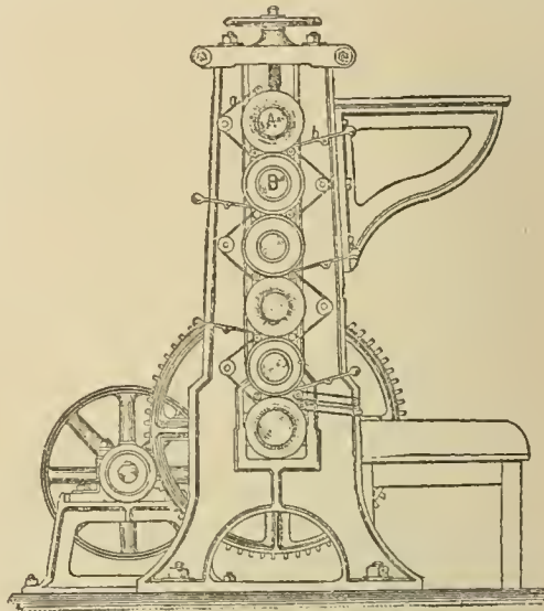
Fig. 11.—Sheet Glazing Calender.
