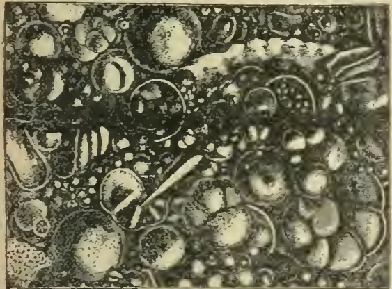
FIG. 2.— Globigerina Ooze from 1900 fathoms.
