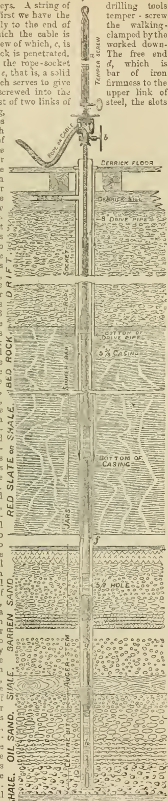
Fig. 1.—String of Tools.
