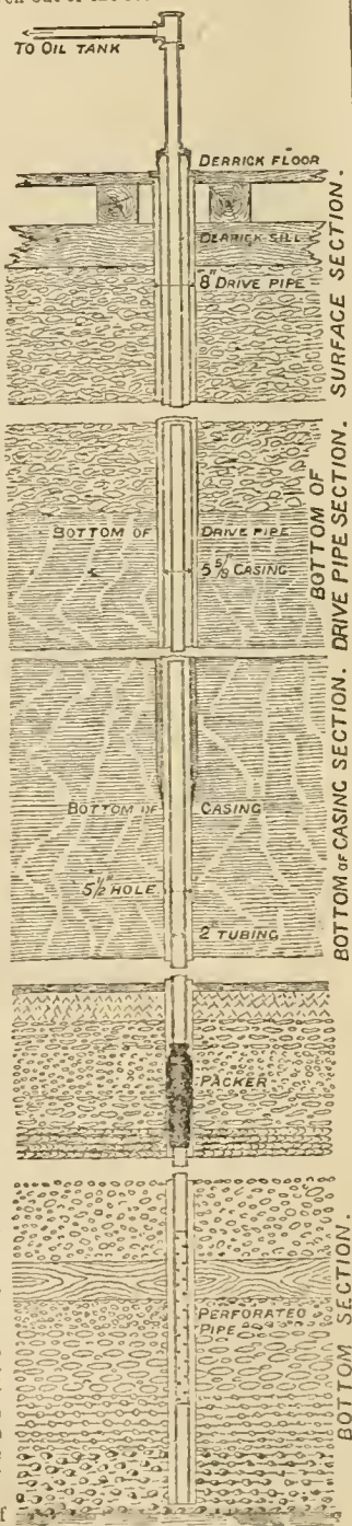
Fig. 3.—Flowing Well.
