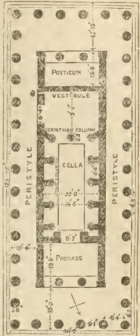
FIG. 1.—Plan of the Temple at Bassæ.
