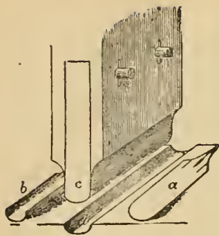
Figure 6. The flat blank a is pushed under the sinker c , is pressed by the action of the lever into the groove d , and comes out with its edges curved up, as in b . The seventh process consists in hardening , which is done by placing the pens in an iron box or muffle , and when they are at a red heat, throwing them into oil; this renders them exceedingly
