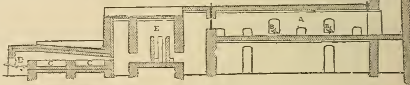
FIG. 14.—Porion Evaporator.
