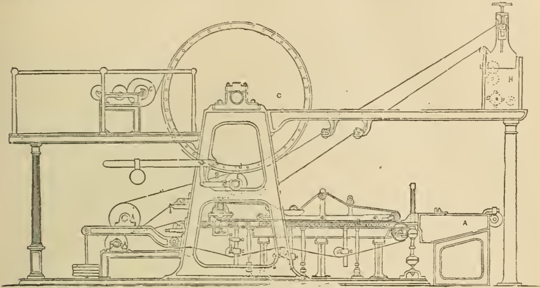
FIG. 6.—Single-Cylinder Machine.
