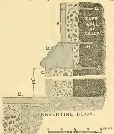
FIG. 5.—Example of marble lining, from the cella of the temple of Concord. A. Slabs of Phrygian marble. B. Plinth moulding of Numidian "giallo." C. Slab of cipollino (Carystian marble). D. Paving of porta santa. E and F. "nucleus" and "rudus" of concrete bedding. G, G. Iron clamps run with lead to fix marble lining. H. Bronze clamp. J. Cement backing.
