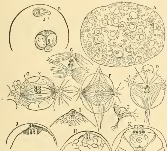
FIG. 11.—Fecundation of ovum (after Van Beneden). A, ovum before entrance of spermatozoon (showing complexity of structure); B, deformation of germinal vesicle on penetration of spermatozoon; C, prothyalosoma with two chromatin disks and axial fibres; D, E, F, later stages of the ypsiform figure; G, second pseudo-karyokinetic figure; H, I, J, K, expulsion of first polar globule.
