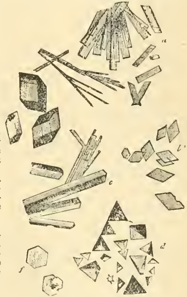
FIG. 9.—Crystals of oxyhemoglobin; a, b, c, e, forms from blood of man and majority of mammals; d, tetrahedral crystals from blood of guinea-pig; f, hexagonal crystals from squirrel's blood.
