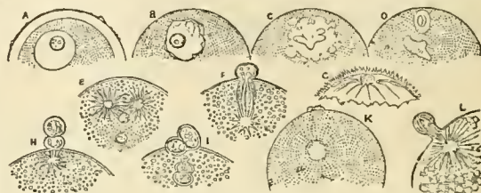
FIG. 10.—A, ripe ovum of Asterias glacialis , with eccentric germinal vesicle and spot; B-E, gradual metamorphosis of germinal vesicle and spot; F, detachment of first polar body and withdrawal of remaining part of nuclear spindle within the ovum; G, portion of living ovum with first polar body; H, formation of second polar body; I, after formation of do., showing the remaining internal half of the spindle in the form of two clear vesicles; K, ovum with two polar bodies and radial striae round female pronucleus; L, expulsion of polar body. (A-K after Fol; L after Hertwig.)
