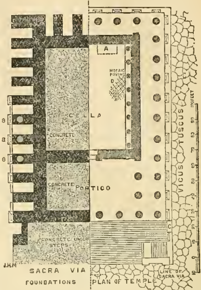
FIG. 14.—Plan of temple of Castor, half showing construction of podium. A. Pedestal of one of the two statues. B, B, B. Spurs of foundation wall, of travertine and tufa, under the three existing columns. C. Steps to small chamber in concrete core of podium. D. Existing piece of mosaic paving of earlier building.
