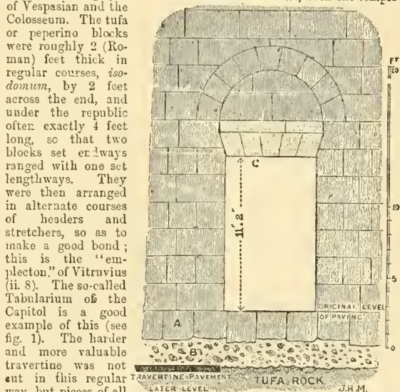
FIG. 1.—Example of opus quadratum , 78 B.C. Arch at foot of the stairs of the Tabularium (see Plate VII.). The flat arch C is of travertine, the rest of peperino. A. Footing-course of rough stones. B. Concrete foundation, exposed by the lowering of the paving when the temple of Vespasian was built.
