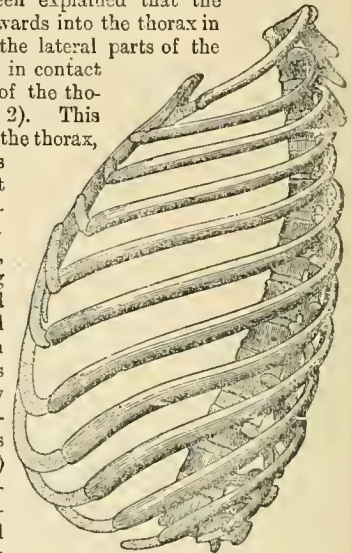
Fig. 5.—Showing slope of ribs. (From Hermann's Handbuch .)
