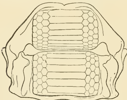
FIG. 4.—Jaws of an Eagle-Ray, Myliobatis aquila .
