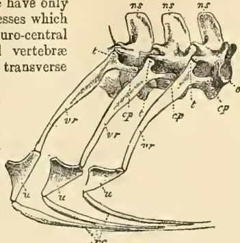
FIG. 4.—Lateral aspect of three thoracic vertebrae of Crocodilus vulgaris (from nature). c, cap on the anterior surface of centrum; cp, capitula of ribs; ns, neural spines; rc, rib cartilages; t, tubercula of ribs; u, unclinate processes; vr, vertebral ribs.
