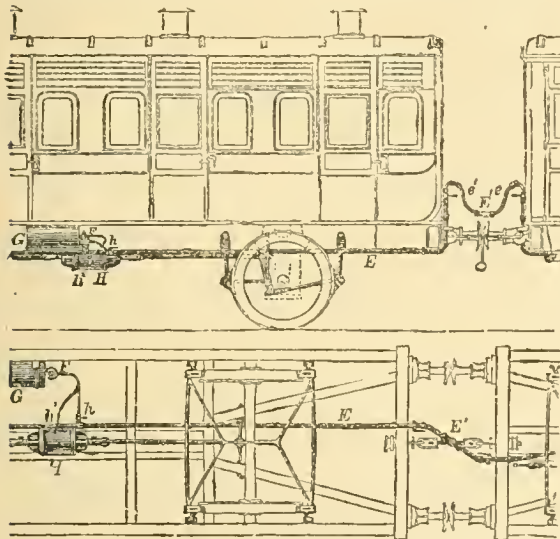
Fig. 44.—E, the brake-pipe, extends the whole length of the train, connected between the vehicles by a coupling E', with flexible pipes c, c; F, the triple valve at the end of the reservoir G; H, the brake-cylinder, with pistons and rods connected with the brake-levers and the blocks suspended on frames; h, a branch pipe from the brake-pipe or main to the triple valve and reservoir; h', a branch pipe from the reservoir and triple valve to the brake-cylinder.
