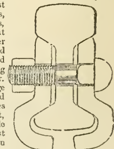
Fig. 33.—Bull-headed rail and fish-plate, Midland Railway.
