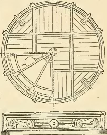
FIG. 22.—Carriage turn-table for stations.
