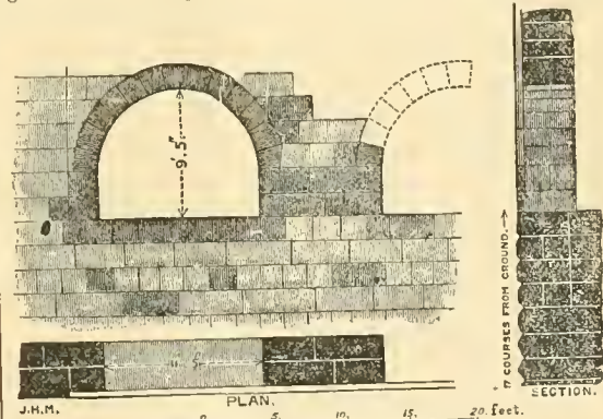
FIG. 8.—Part of Servian wall on Aventine.
