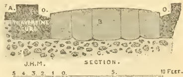
FIG. 6.—Example of early basalt road by the temple of Saturn on the Clivus Capitolinus. A. Travertine paving. B. Polygonal basalt blocks. C. Concrete bedding. D. Rain-water gutter. The curb shown is taken from another part of the road.
