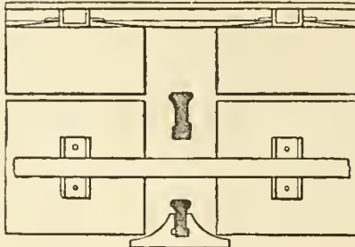
FIG. 3.—The fish-belly rail, 1820-30.
