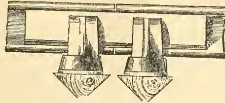
FIG. 9.—The original fish-joint, by W. Bridges Adams.
