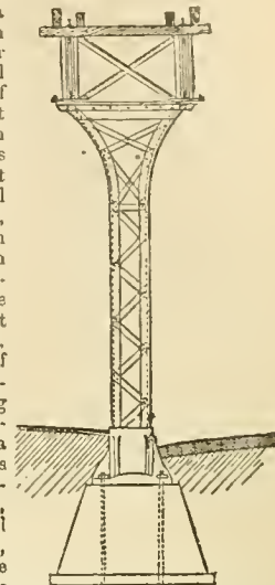
Fig. 27.—New York Elevated Railroad. Square lattice-work column.
