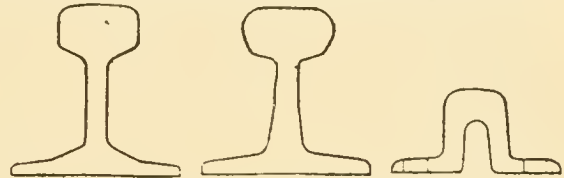
FIG. 35.—Flange rail; New South Wales Railway. FIG. 36.—Flange rail; Midland Great Western Railway. FIG. 37.—Bridge rail; Great Western Railway.
