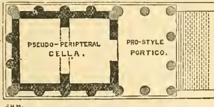
FIG. 21.—So-called temple of Fortuna Virilis. The black shows tufa; the shading travertine.
