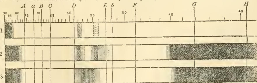
FIG. 10.—1, 2, Spectra of solutions,—1 containing less than 0.01 per cent. and 2 containing 0.07 per cent. of oxyhemoglobin; 3, spectrum of solution containing about 0.2 per cent. of hemoglobin.
