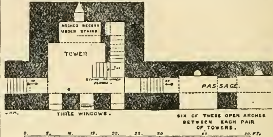
FIG. 25.—Aurelian wall; plan showing one of the towers and the passage in thickness of wall.
