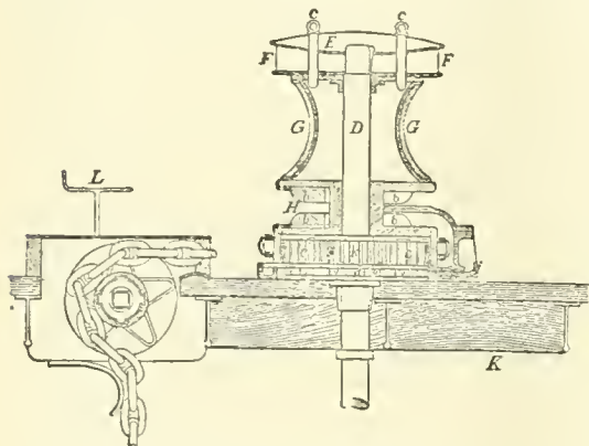
FIG. 1.—Vertical Section of Capstan.
