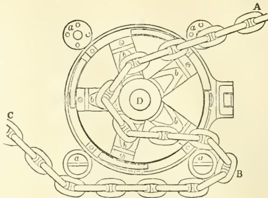
FIG. 2.—Plan of Capstan
