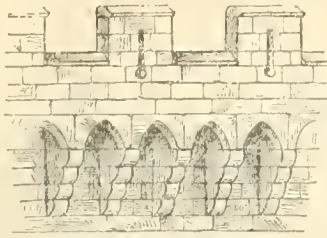
FIG. 3.—Machicolations and Battlemented Parapet.
