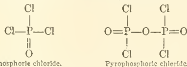
Phosphoric chloride.
