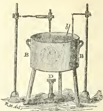
FIG. 8.—Dumas's Vapour-density Apparatus. A, glass globe, supported by wire claw; b, projecting portion of neck; BB, bath; C, thermometer; D, gas-burner for heating bath.
