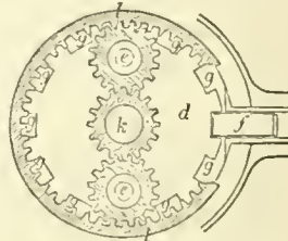
FIG. 3.—Section showing Pinions.
