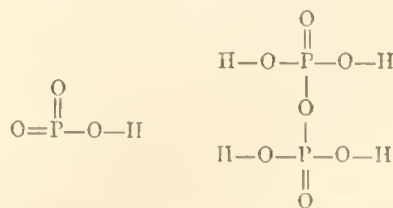
Meta-phosphoric acid.
