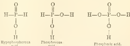
Hypophosphorous acid.
