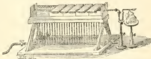
FIG. 5.—Apparatus arranged for a Combustion.
