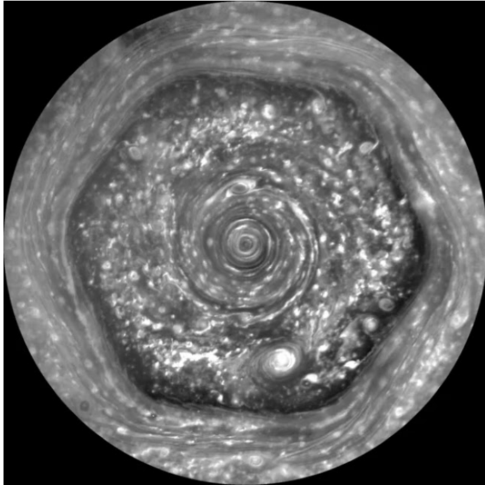
Hexagon on Saturn's North Pole. One can draw a 3D cube in this 2D Hexagon.
