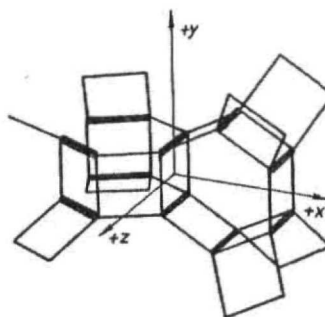
Hilgenberg's Krypton Model (Number 26, Mass 82)
