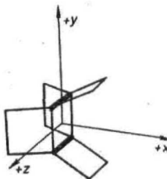
Hilgenberg's Neon Model (Number 10, Mass 22)
