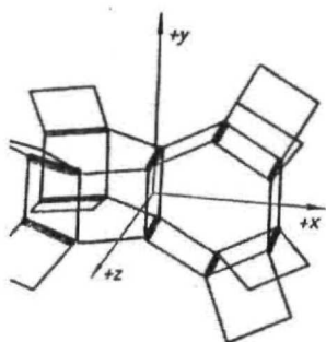
Hilgenberg's Krypton Model (Number 26, Mass 82)
