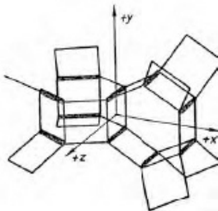
Hilgenberg's Krypton Model (Number 26, Mass 82)
