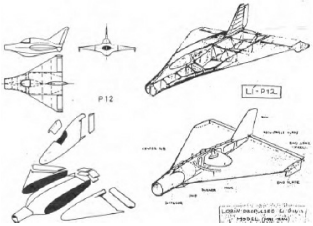
Lippisch's P-12 Design
