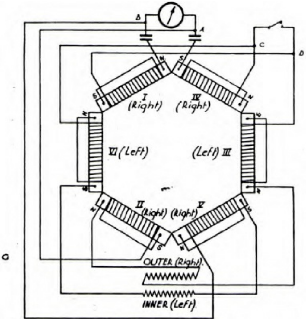
The Coler Coil
