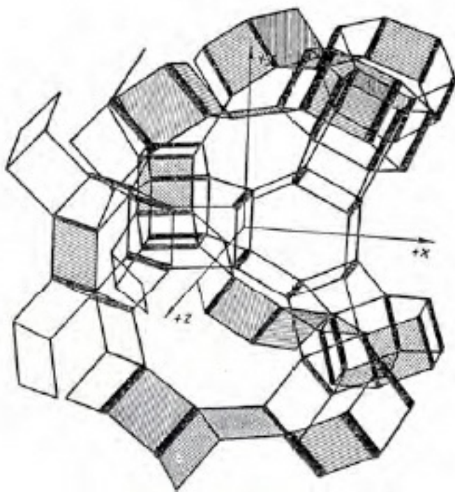
Hilgenberg's Model of Element 118, Mass 336
