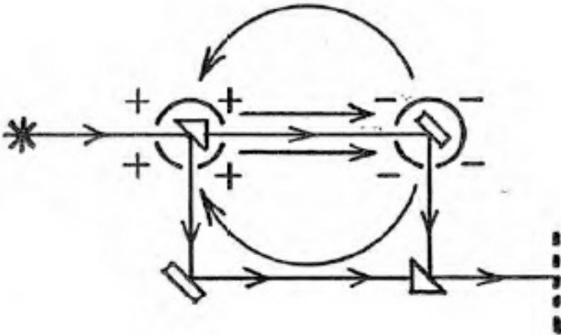
Krafft's Interferometer
