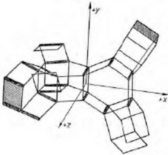
Hilgenberg's Xenon Model (Number 54, Mass 132)
