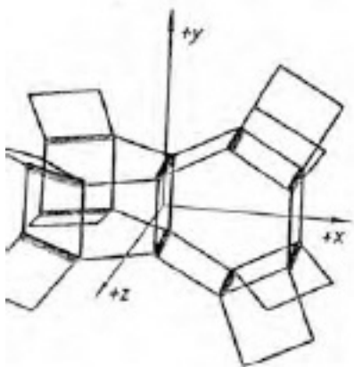
Hilgenberg's Krypton Model (Number 26, Mass 82)
