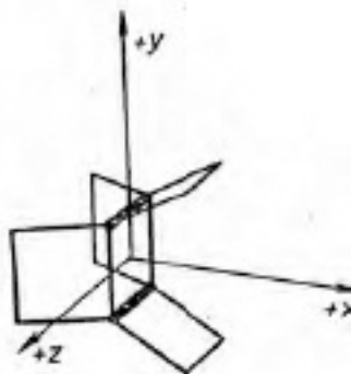
Hilgenberg's Neon Model (Number 10, Mass 22)
