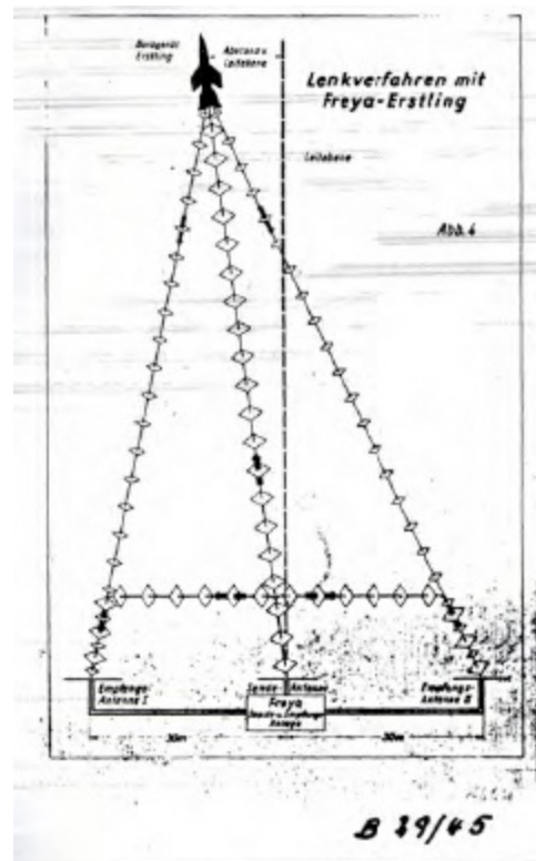
Schematic of the Envisioned Use of Freya for Rocket Guidance
