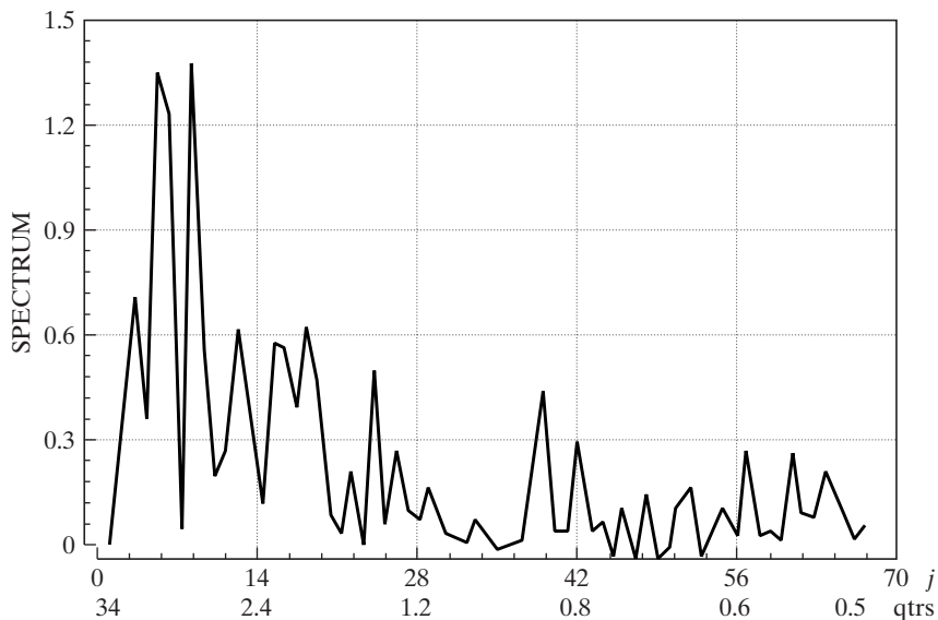
FIGURE 20.3 Sample Periodogram.
