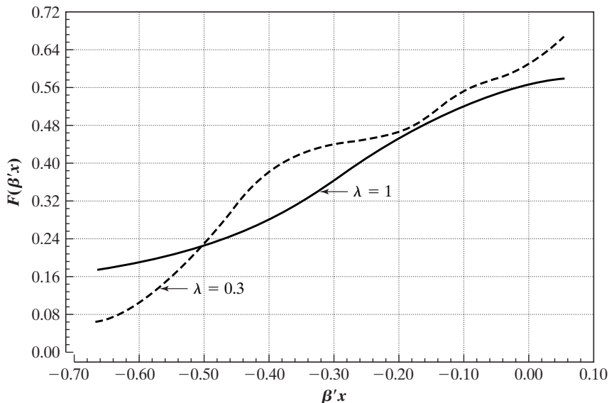
FIGURE 21.3 Nonparametric Regression.
