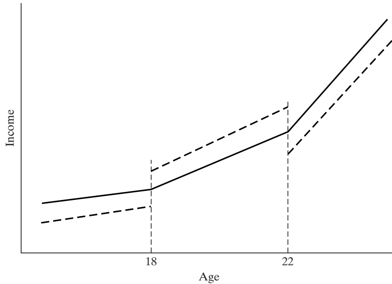
FIGURE 7.2 Spline Function.
