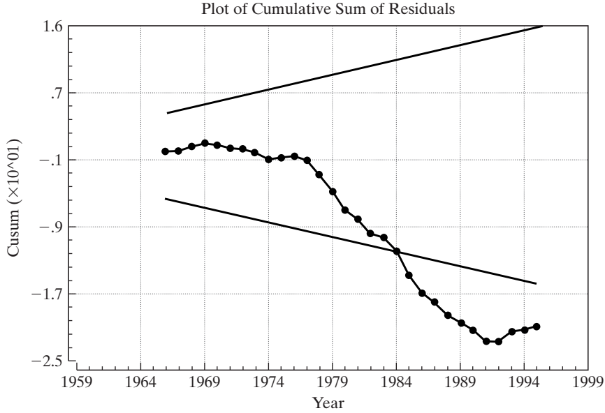
FIGURE 7.6 CUSUM Test.
