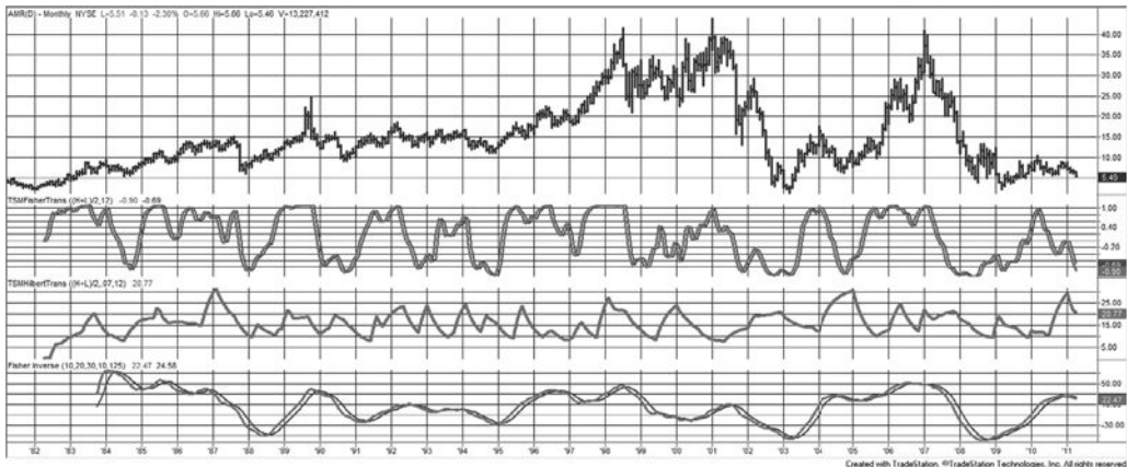
FIGURE 11.22 Monthly AMR (top) prices from 1982 with the Fisher Transform (2nd panel), Hilbert Transform (3rd panel), and Inverse Fisher Transform (lower panel)
