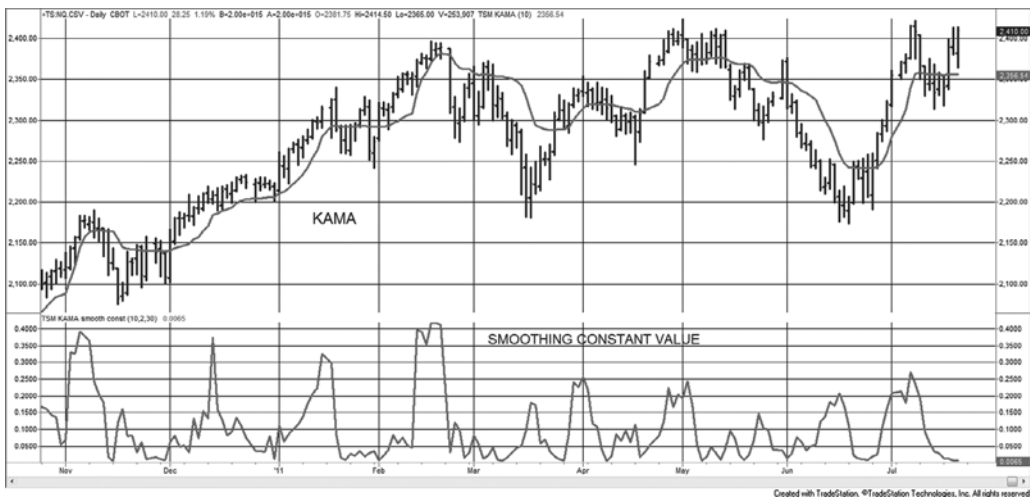
FIGURE 17.2 Kaufman’s Adaptive Moving Average and the smoothing constant values on each day, emini NASDAQ futures, November 2010 to July 2011.
