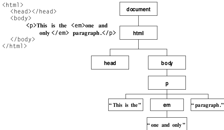
Figure 4-12: A simple HTML document node tree.
