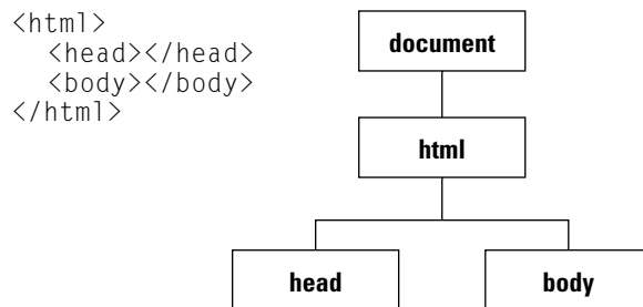
Figure 4-8: Object map of an empty document.
