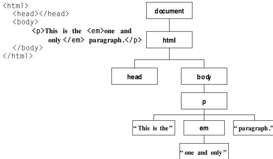
Figure 4-11: Inserting an element into a text node.
