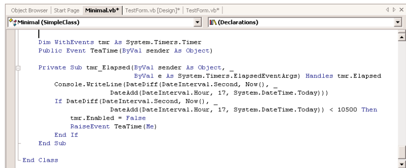
FIGURE 8.7 Declaring and raising an event in the class's code
