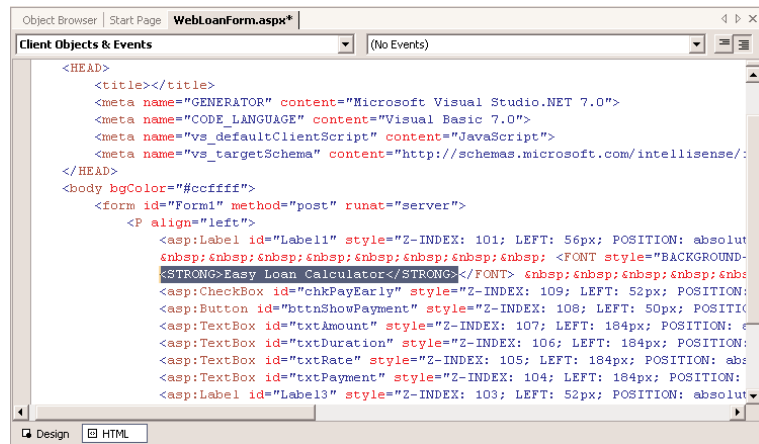
FIGURE 2.9 Editing the Web form’s HTML code
