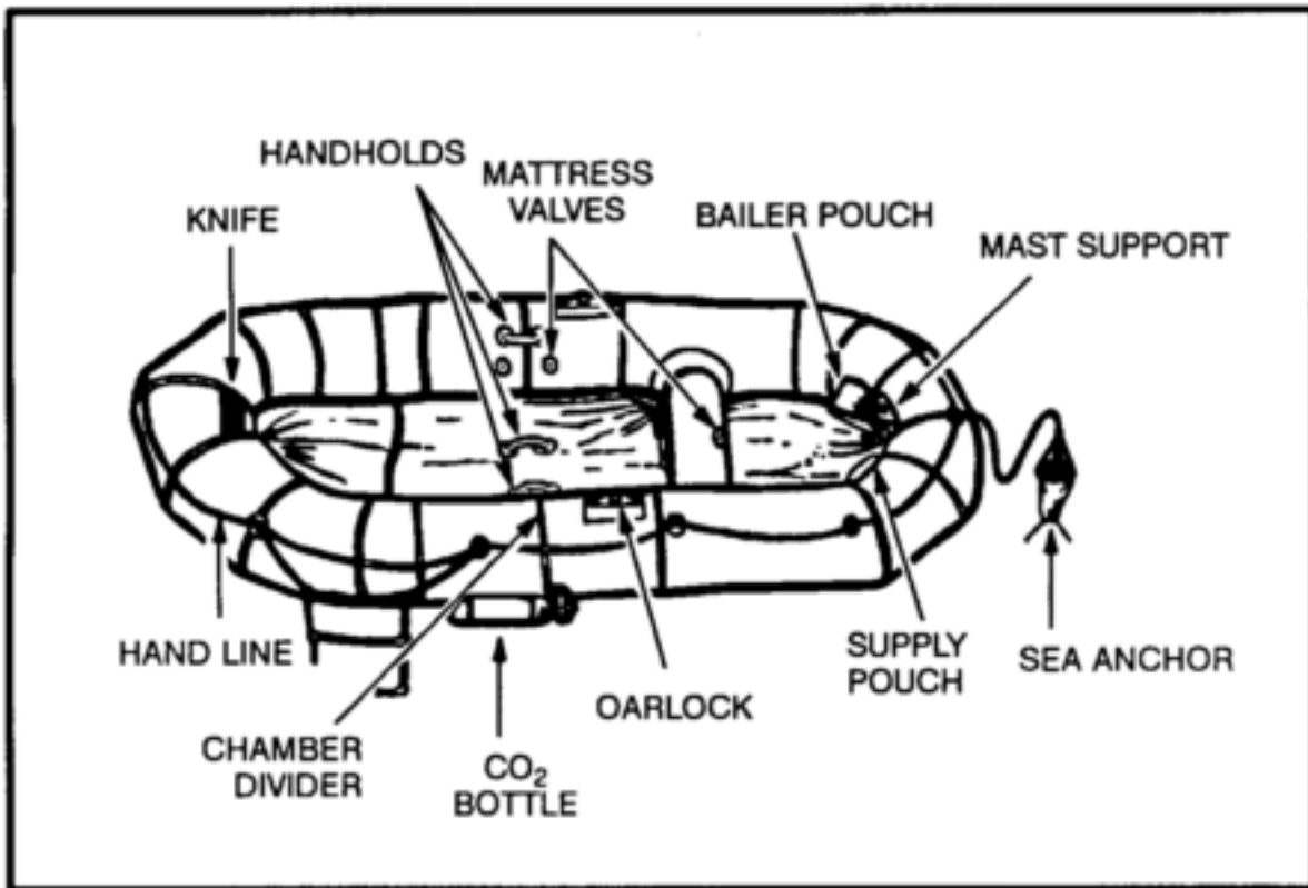
Figure 16-12. Seven-man raft.
