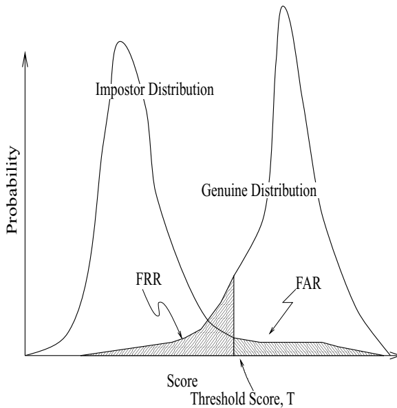
Figure 8.23 Probability distributions of matcher scores from genuine mated and impostor fingerprint pairs. FRR and FAR denote the false reject and false accept error rates, respectively.
