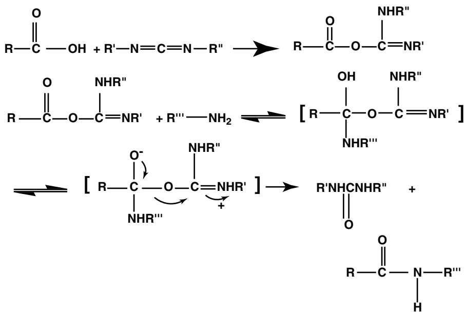
Figure 6.17 Carbodiimide-mediated amidation reaction.
