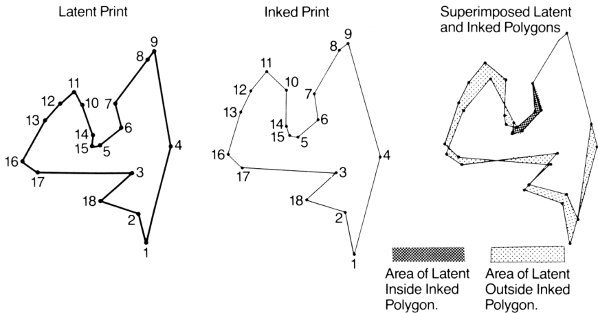
Figure 2.3 Polygon method.
