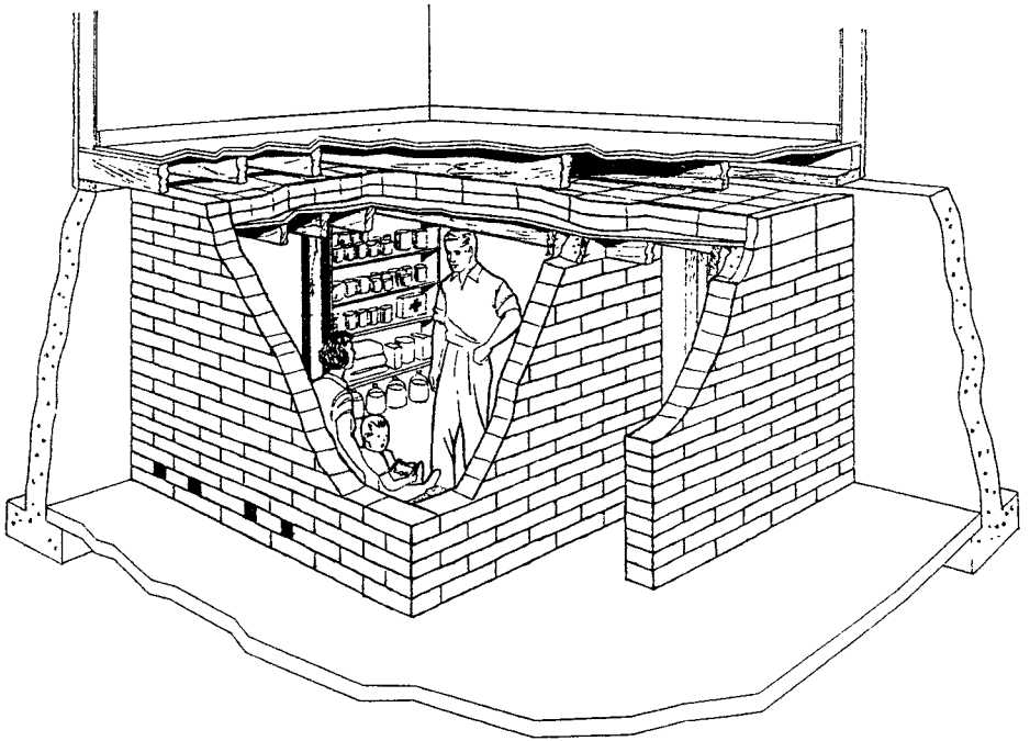
Figure 7—Basement Concrete Block Shelter
