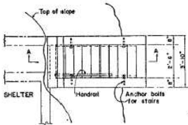
PLAN (Door Removed)
