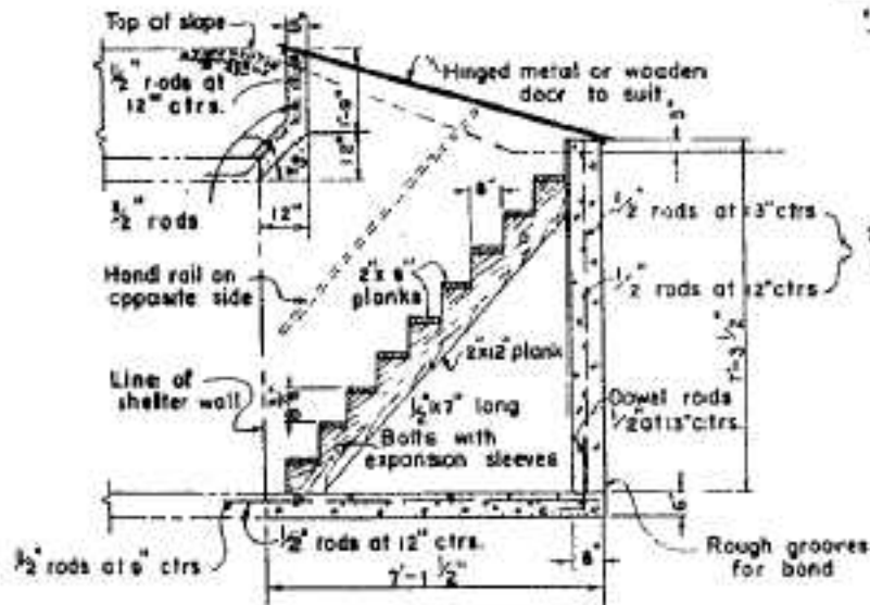
SECTION A-A ALTERNATE STAIRWAY DETAILS
