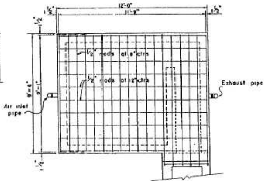
ROOF PLAN SHOWING REINFORCING
