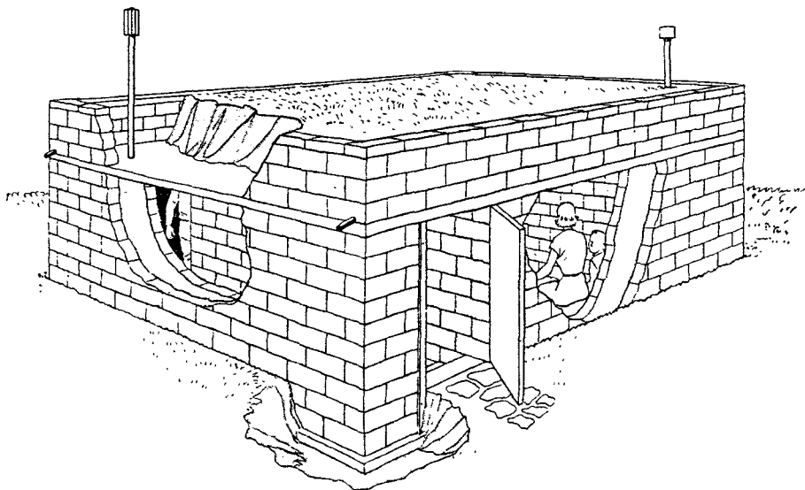
Figure 9.—Aboveground double-wall shelter
