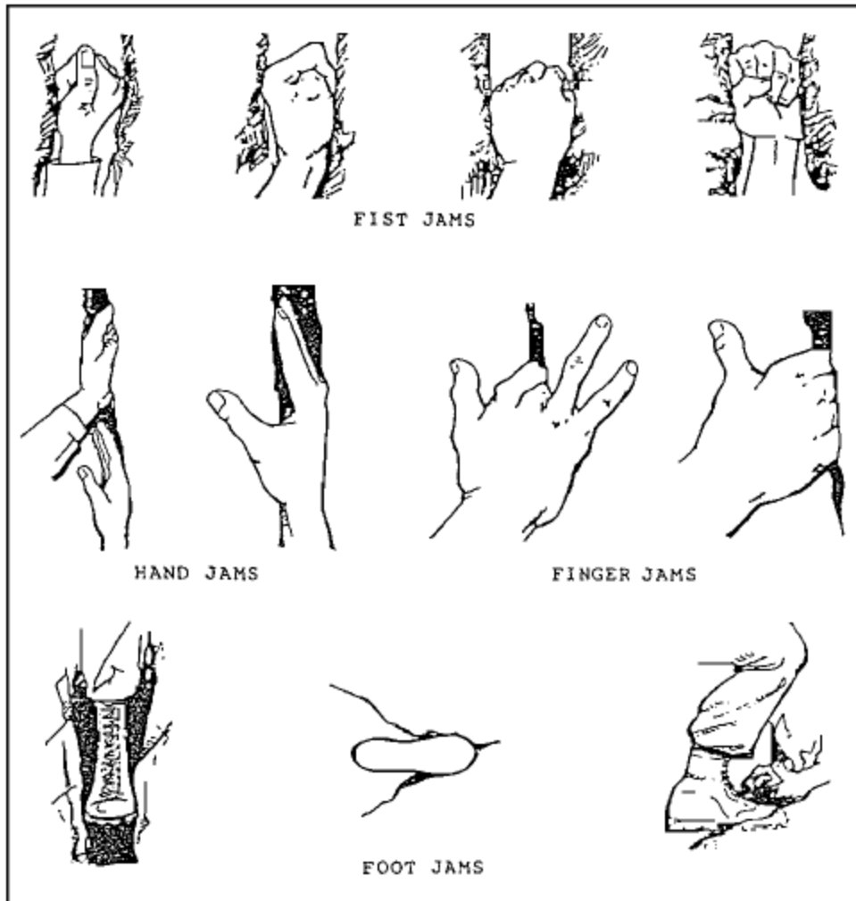
FIGURE 3-7. Jam Holds.
