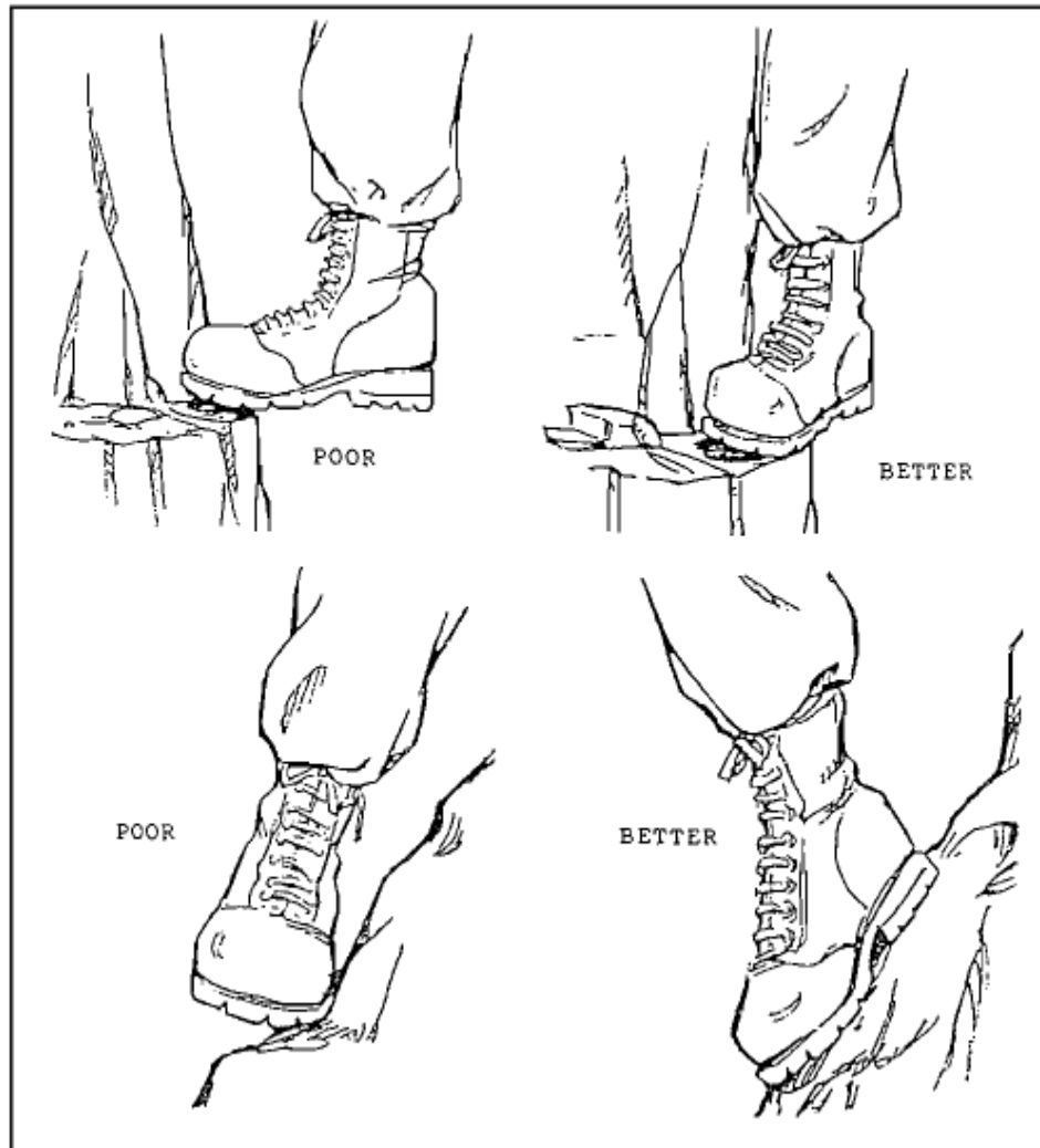
FIGURE 3-8. Footholds
