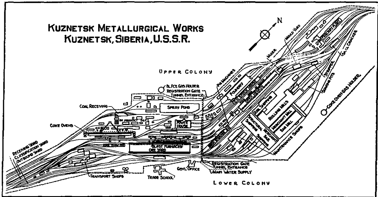
Figure 16-1 LAYOUT OF KUZNETSK IRON AND STEEL PLANT PREPARED BY FREYN ENGINEERING COMPANY UNDER TECHNICAL-ASSISTANCE CONTRACT OF 1930
