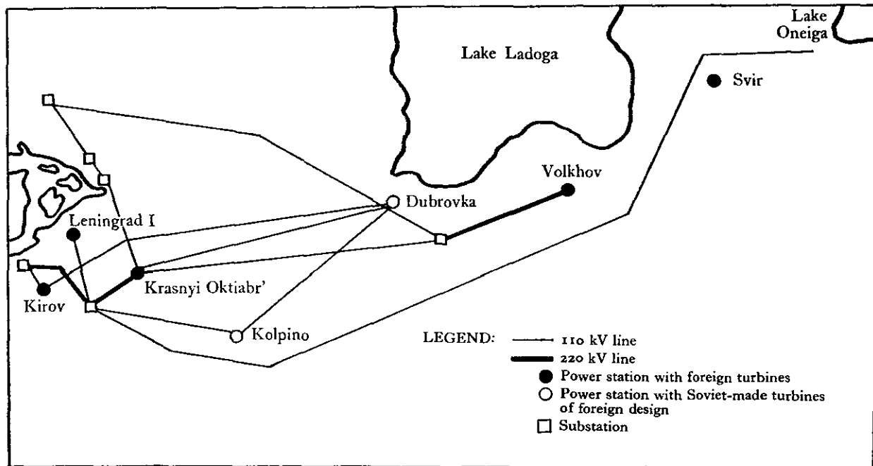
Figure 10-3 ORIGIN OF STEAM AND HYDRAULIC TURBINES IN THE LENINGRAD GRID SYSTEM, 1930-44
