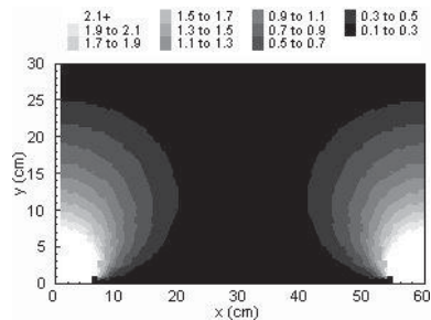
Ex-field distribution
