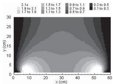
Ey-field distribution
