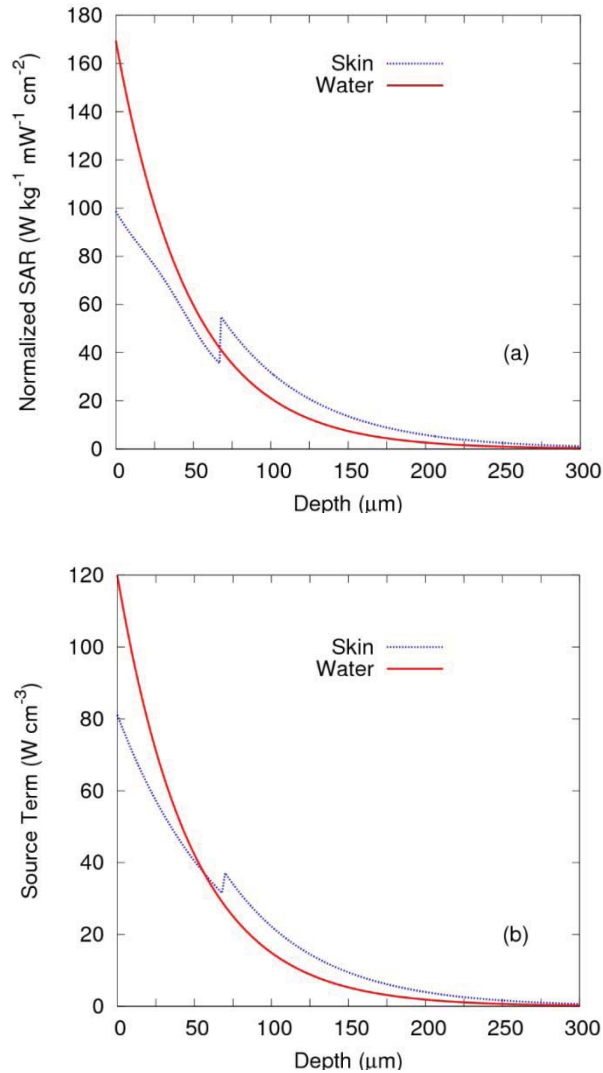
Figure 13-2. Axial distribution of the source term (a) Normalized SAR (b) Linear Absorption, for two-layer skin model and water for a 1\text{-}W\text{cm}^{-2} , 1-THz exposure along r = 0 .
