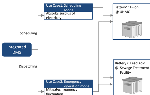
Figure 6 Controlling distributed bulk battery energy storage
