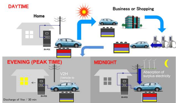
Figure 23 Assumed EV charge and discharge in V2G Program
