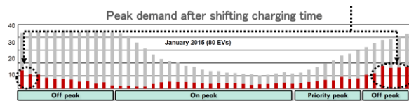
Figure 21 State of charging of all EVs after implementing charging management
