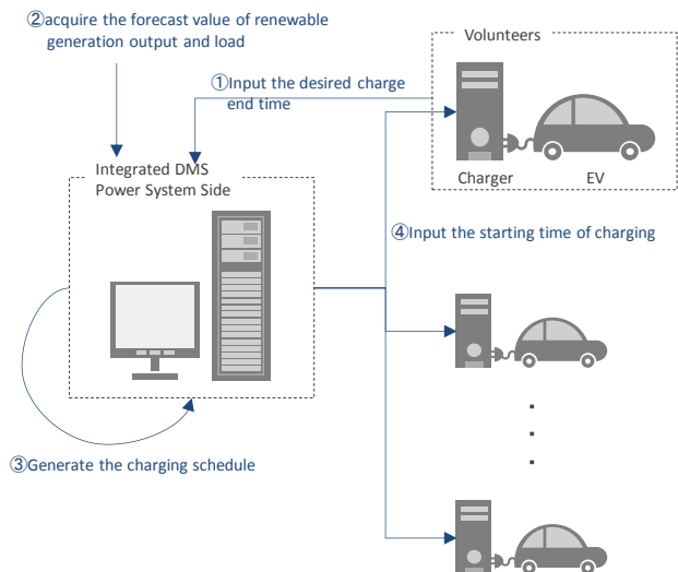
Figure 18 Structure of Charging Management Program
