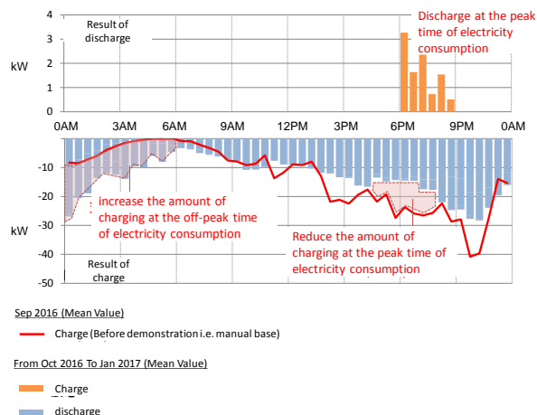
Figure 24 Charging and discharging of EV in V2G Program
