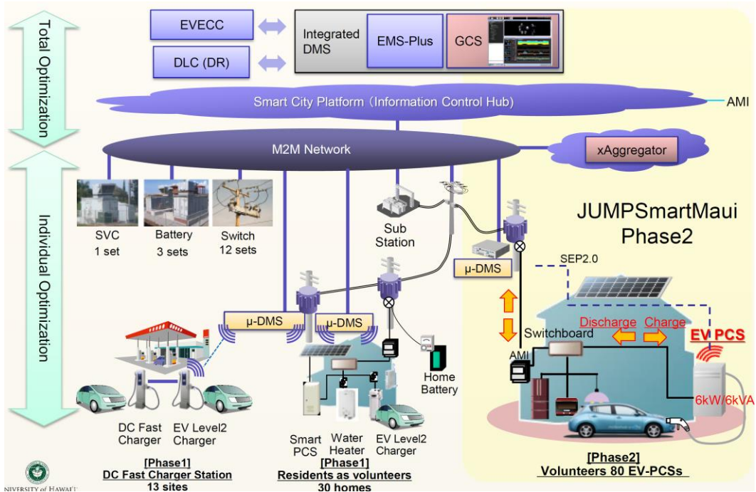
Figure 3 Overall structure of JUMPSmartMaui Smart Community System
