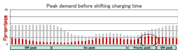
Figure 20 State of charging of all EVs before implementing charging management
