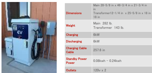
Figure 22 Specifications of EV-PCS
