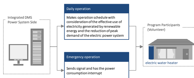
Figure 5 Structure of Direct Load Control program
