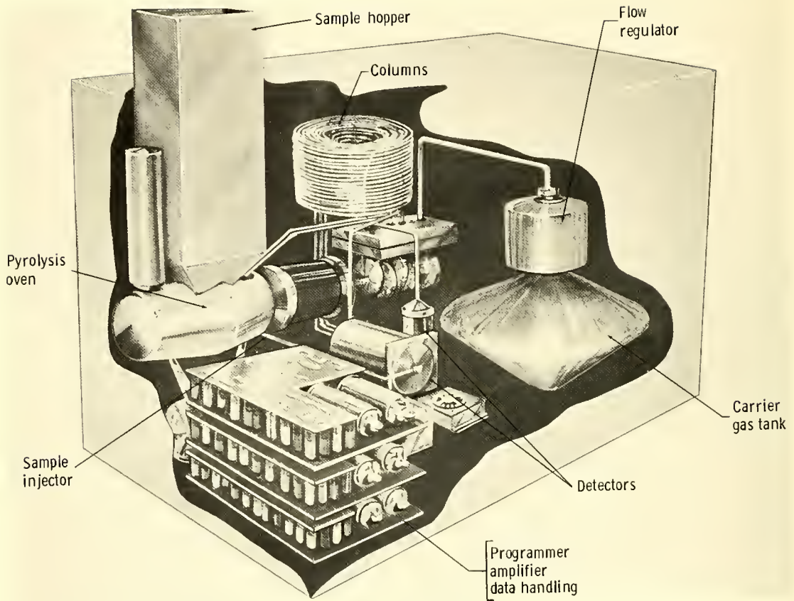
FIGURE 5.—Gas chromatograph.
