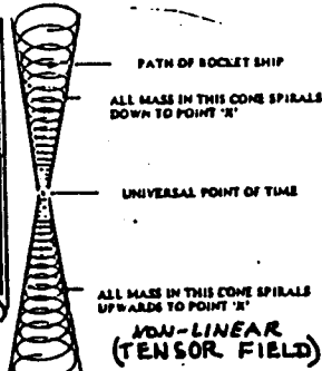
Fig. 13. General Relativity The Space-Time Diagram. (Time-Cone)
