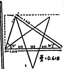
Fig. 11. Origin of \Phi in 5-Point Star.
