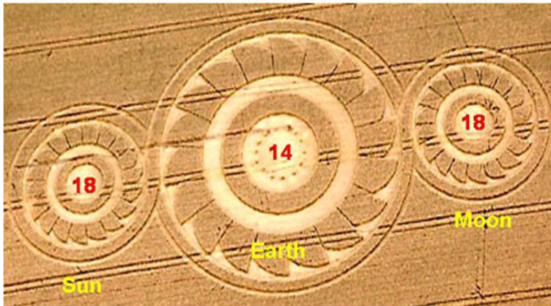
The 18-year Saros eclipse cycle portrayed as "three meshing gears": a lunar eclipse 14 days later on August 16, 2008
