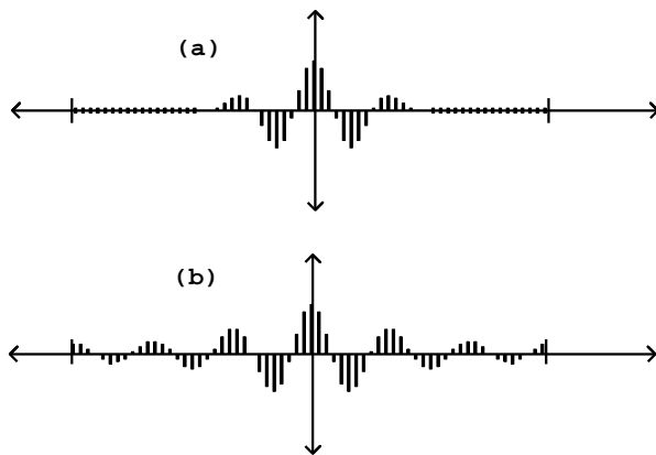
Figure 6.5: Audio signals resulting from multiplying a cosine (partial number 6) by pulse trains: (a). windowing function from the wavetable formulation; (b) wavelookup output using the Gaussian lookup function.
