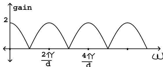
Figure 7.6: Gain of the delay network of Figure 7.3, shown as a function of angular frequency \omega .
