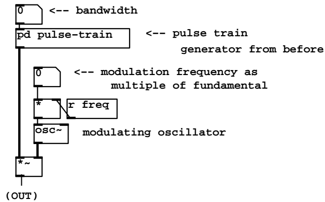
Figure 6.14: Excerpts from patch example F05.ring.modulation.pd combining ring modulation with a stretched wavetable pulse generator
