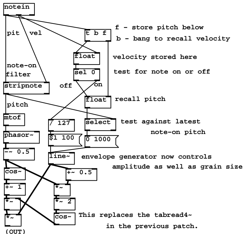
Figure 3.16: A MIDI-style monophonic synthesizer.
