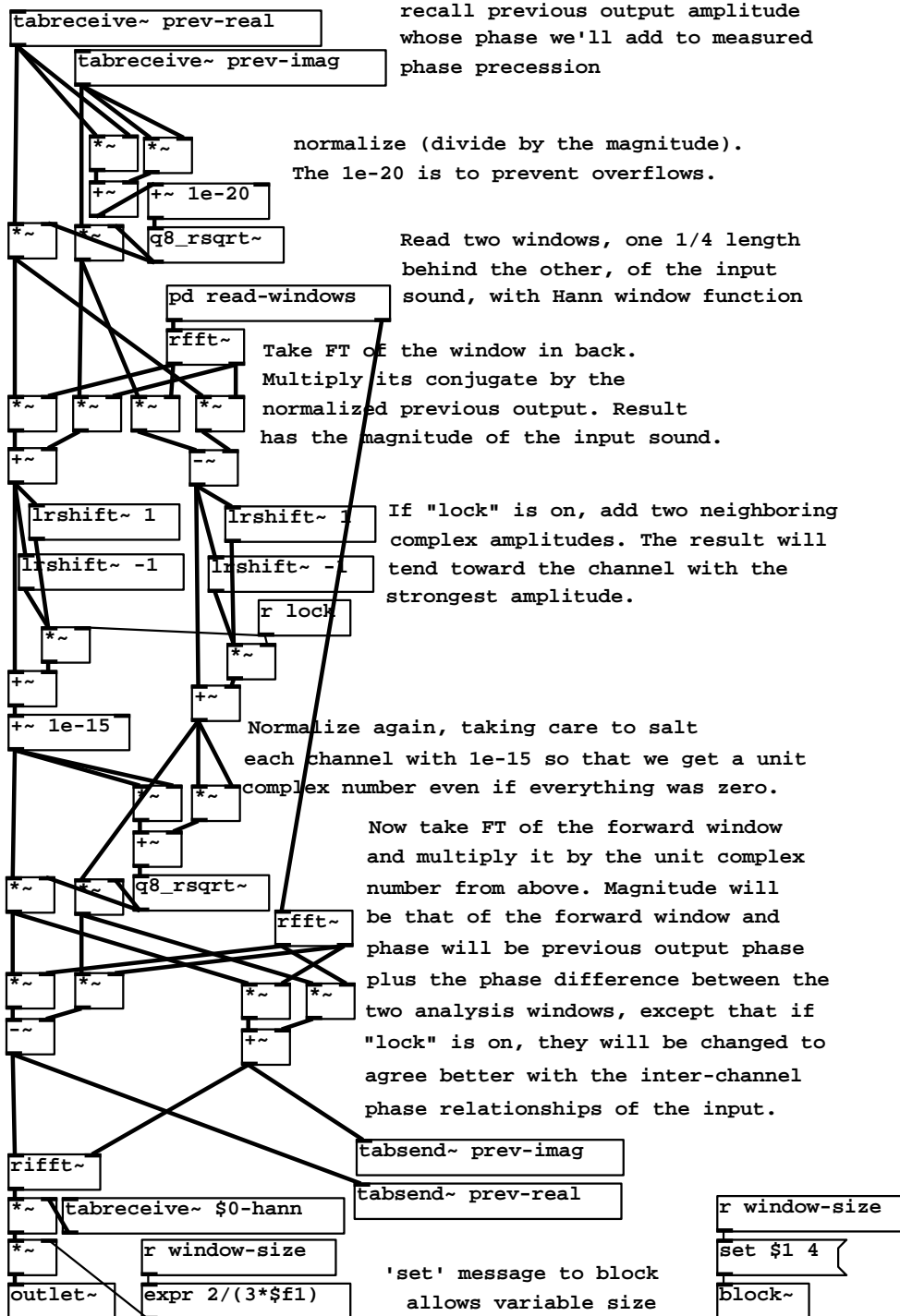
Figure 9.18: Phase vocoder for time stretching and contraction.
