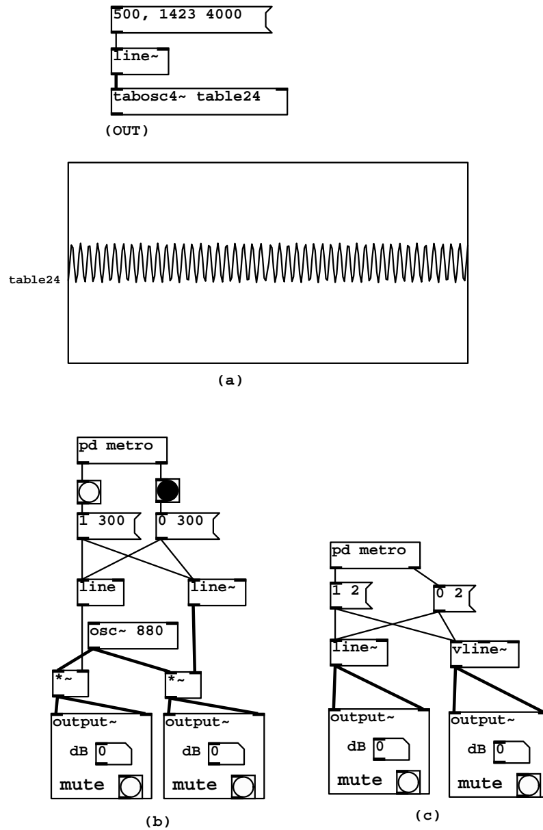
Figure 3.13: Sending an oscillator over the Nyquist frequency.
