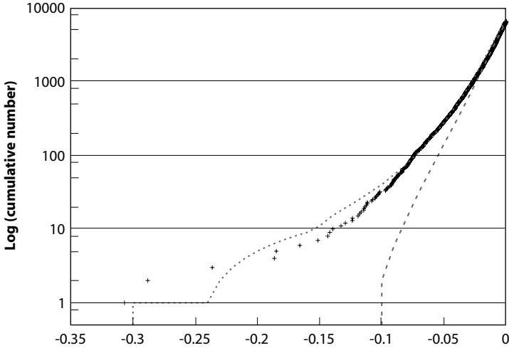
FIG. 3.7. The two dashed lines are defined such that 99% of the drawdowns of synthetic GARCH(1,1) with noise Student distribution with 4 degrees of freedom are within the two lines. The symbols + represent the cumulative distribution of the drawdowns for the DJIA. The ordinate is in logarithmic scale, while the abscissa shows the drawdowns; for instance, -0.30 corresponds to a drawdown of -30\% . Reproduced from [399].
