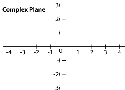
FIG. 6.16. Complex plane: The horizontal line represents the real numbers, which include in particular the integers -3, -2, -1, 0, 1, 2, 3, \dots . The vertical line represents the purely imaginary numbers, products of i by arbitrary real numbers. The rest of the plane is the set of nonreal complex numbers. The terms “complex” and “imaginary” are suggestive of the fact that these numbers lie above the real numbers and are observed as projections or “shadows” on the real axis.
