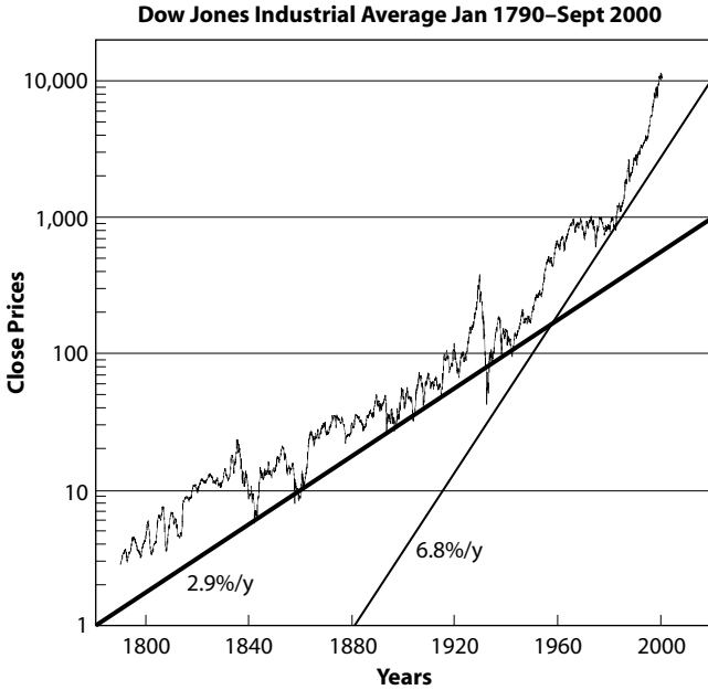
FIG. 2.1. Monthly quotes of the DJIA from September 2000 extrapolated back to January 1790. The vertical axis uses logarithmic scales such that multiplication by a fixed factor, for instance 10, corresponds to addition of a constant in this representation. Mathematically, this corresponds to a mapping from multiplication to addition and allows us to show on the same graph prices that have changed by factors of thousands (in the present case, from a value of about 3 in 1790 to a value above 10,000 in 2000). The thick (respectively, thin) straight line corresponds to the exponential growth of an initial wealth of $1 in 1780 (respectively, 1880) invested at the annual rate of return of \approx 2.9\% (respectively, 6.8\% ), which would have transformed into $1,000 (respectively, $10,000) in 2020.
