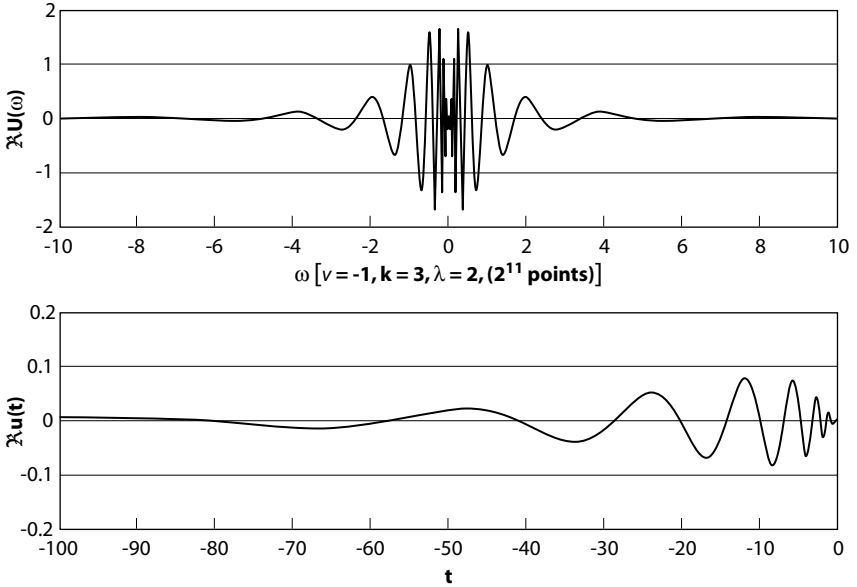
FIG. 6.23. Typical waveform of an Altes wavelet, a mathematical function exhibiting log-periodic symmetry, used by bats and dolphins to optimize their ultrasonic signals. The upper panel shows the Fourier transform as a function of angular frequency of the Altes wavelet represented in the lower panel as a function of time. Recall that the Fourier transform of a signal is nothing but the quantification of the sinusoidal components constituting the signal. Notice that both the Altes wavelet and its Fourier transform exhibit log-periodic oscillations.
