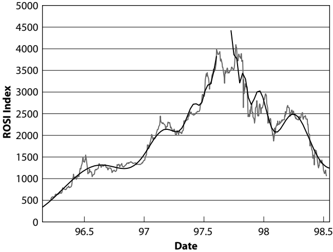
Fig. 8.33. Symmetric “bubble” and “antibubble”: in addition to the ascending part of the ROSI Index, which is reproduced from Figure 8.32 with the same fit, we show the deflating part fitted with equation (15) by changing t_c - t into t - t_c . The parameter values are A_2 \approx 4922 , B_2 \approx -3449 , B_2 C \approx 472 , m_2 \approx 0.32 , t_c \approx 97.72 , \phi \approx 1.4 , and \omega \approx 7.9 . Reproduced from [221].
