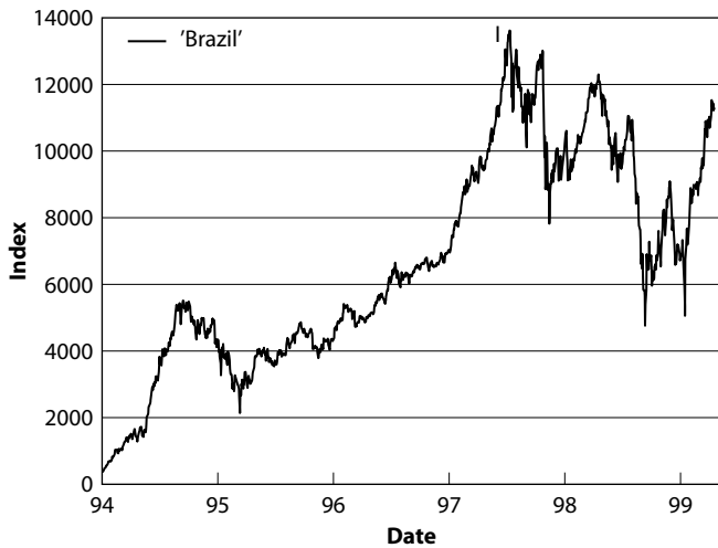
FIG. 8.2. The Brazilian stock market index as a function of time. One bubble with a subsequent very large drawdown can be identified. The approximate date is mid-97 (I). Reproduced from [218].
