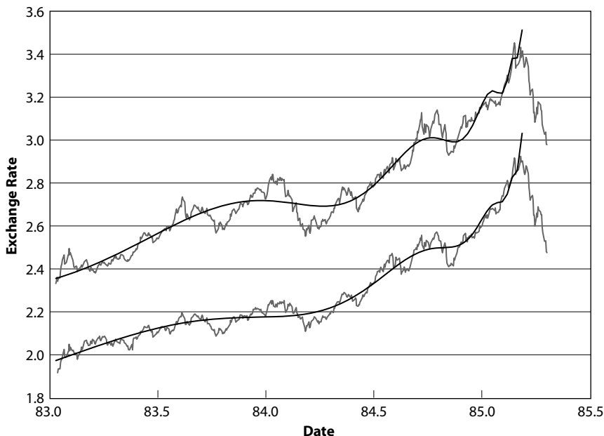
FIG. 7.15. The U.S. dollar expressed in German Mark DEM (top curve) and in Swiss franc CHF (bottom curve) prior to its collapse on mid-1985. The fit to the DEM currency against the U.S. dollar with equation (15) is shown as the continuous and smooth line and gives A_2 \approx 3.88 , B_2 \approx -1.2 , B_2C \approx 0.08 , m_2 \approx 0.28 , t_c \approx 1985.20 , \omega \approx 6.0 , and \phi \approx -1.2 . The fit to the Swiss franc against the U.S. dollar with equation (15) gives A_2 \approx 3.1 , B_2 \approx -0.86 , B_2C \approx 0.05 , m_2 \approx 0.36 , t_c \approx 1985.19 , \omega \approx 5.2 , and \phi \approx -0.59 . Note the small fluctuations in the value of the scaling ratio 2.2 \leq \lambda \leq 2.7 , which constitute one of the key tests of our “critical herding” theory. Reproduced from [212].
