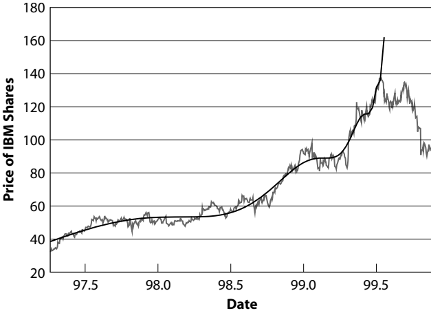
FIG. 7.23. Best (r.m.s. \approx 3.7 ) fit, shown as solid line, with equation (15) to the price of IBM shares. The parameter values of the fits are A_2 \approx 196 , B_2 \approx -132 , B_2C \approx -6.1 , m_2 \approx 0.24 , t_c \approx 99.56 , \omega \approx 5.2 , and \phi \approx 0.1 . Reproduced from [217].
