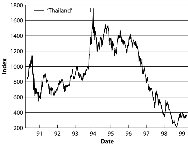
FIG. 8.25. The Thai stock market index as a function of time. One bubble with a subsequent very large drawdown occurring early in 1994 can be identified. Reproduced from [218].
