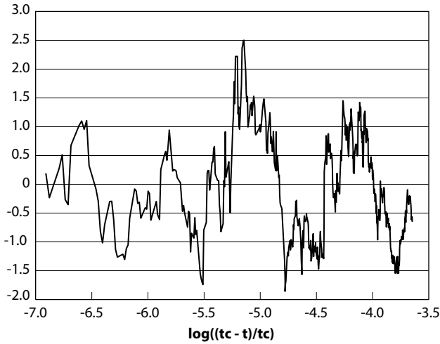
FIG. 7.19. The residual as defined by the transformation explained in the text as a function of \log\left(\frac{t_c - t}{t_c}\right) for the October 1987 crash. Reproduced from [221].
