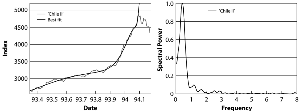
FIG. 8.13. Left panel: The Chilean bubble of 1993. See Table 8.1 for the main parameter values of the fit. Right panel: Lomb periodogram of the oscillatory component of the market price shown in the left panel. Reproduced from [218].
