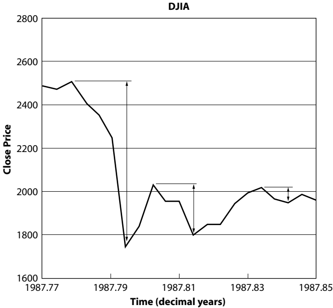
FIG. 3.1. Definition of drawdowns. Taking the example of the crash that occurred on October 19, 1987, this figure shows three drawdowns corresponding to cumulative losses from the last maximum to the next minimum of the price. The largest drawdown of a total loss of -30.7\% is made of four successive daily drops: on October 14, 1987 (1987.786 in decimal years), the DJIA index is down by 3.8\% ; on October 15, the market is down 6.1\% ; on October 16, the market is down 10.4\% . The weekend passes and the drop on Black Monday October 19, 1987 leads to a cumulative loss or drawdown of 30.7\% . In terms of consecutive daily losses, this correspond to the series 3.8\% , 2.4\% , 4.6\% , and 22.6\% (note that returns are not exactly additive, since they are price variations normalized by the price, which itself varies).
