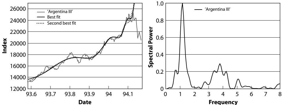
Fig. 8.9. Left panel: The Argentinian stock market bubble ending in 1994. See Table 8.1 for the main parameter values of the fit. Right panel: Only the best fit is used in the Lomb periodogram. Reproduced from [218].
