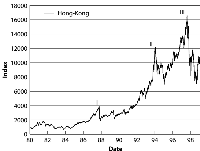
FIG. 7.8. The Hong Kong stock market index as a function of time. Three extended bubbles followed by large crashes can be identified. The approximate dates of the crashes are October 87 (I), January 94 (II), and October 97 (III). Reproduced from [218].
