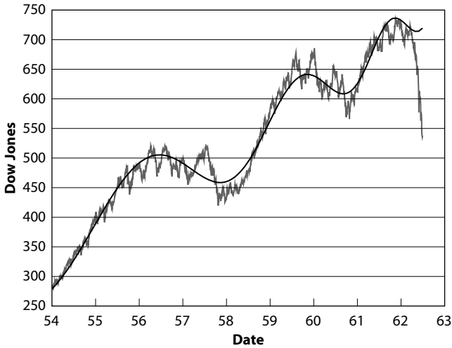
FIG. 7.21. The DJIA prior to the 1962 slow “crash” on Wall Street. The fit (solid line) is equation (15) with A_2 \approx 960 , B_2 \approx -120 , B_2C \approx -14.9 , m_2 \approx 0.68 , t_c \approx 1964.83 , \omega \approx 12.1 , and \phi \approx 4.1 . Reproduced from [209].
