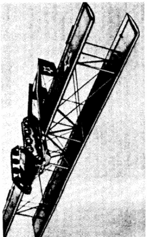
Winged tank KT-1, alias A-40 (Antonov-40), in the air. Pilot S. Anokhin at the controls. Taken from Soviet Tanks and Combat Vehicles of World War Two by Steven J. Zaloga and James Grantzen, Arms and Armour Press, London (1974).
