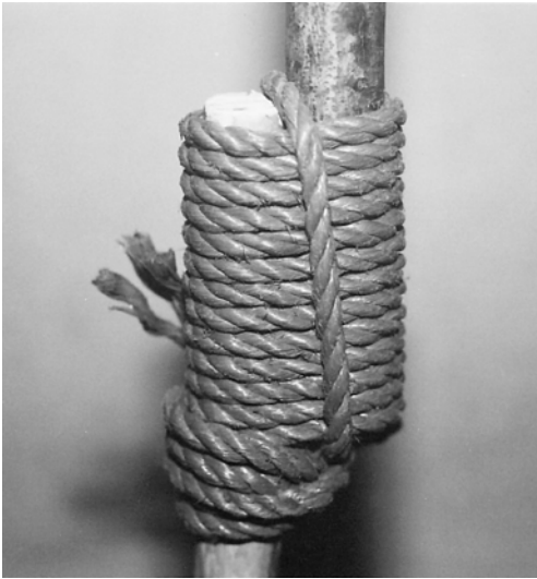
Figure 5.20 Close-up of a forked shaft lashed tightly to a central shaft
