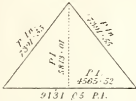
Direct Vertical Section of Gr Pyr.
