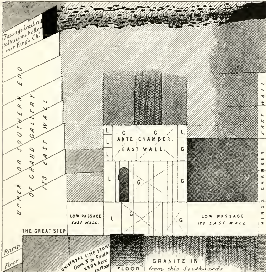
VERTICAL MERIDIAN SECTION from Gr Gallery through ANTE-CHAMBER to Kings Ch. Looking Eastward
