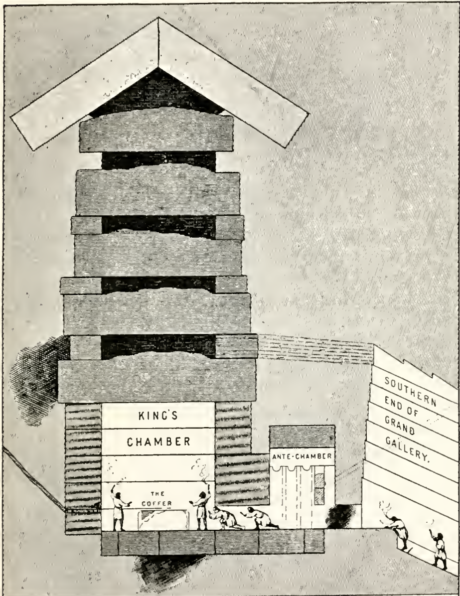
VERTICAL SECTION ( Looking West ) of KING'S CHAMBER: ALSO OF ANTE-CHAMBER, SOUTH END OF GRAND GALLERY, AND VYSE'S HOLLOWES OF CONSTRUCTION, ABOVE KING'S CHAMBER. CROSSED LINES INDICATE GRANITE.
