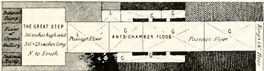
HORIZONTAL SECTION 25 inches above floor or PLAN of FLOOR from Gr Gallery through ANTE-CHAMBER to Kings Ch. Single line shading-Lime stone. Crossed line shading-Granite. Also L Lime stone and G Granite
