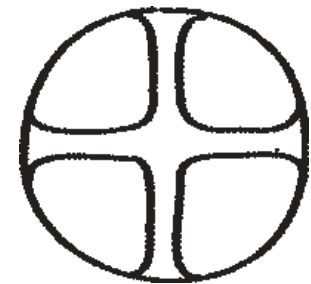
Fig. 2-15. Coptic symbol
