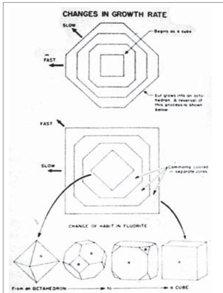
Fig. 6-36. A fluorite crystal.
