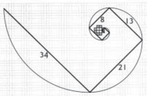
Fig. 8-6. A view of the Fibonacci spiral, both male (straight line) and female (curved).
