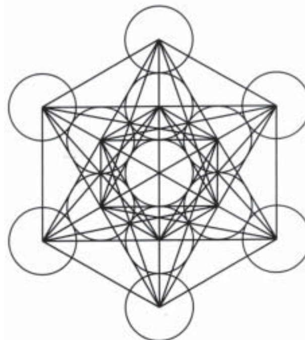
Fig. 7-21. Metatron's Cube.
