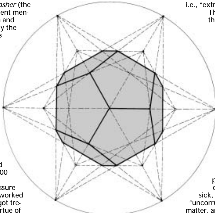
Dodecahedron (in grey)
