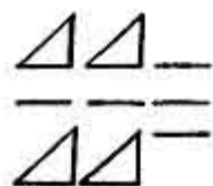
Power of waters
