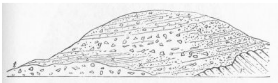
TILL OVERLAID WITH BOWLDER-CLAY, RIVER STINCHAR.
