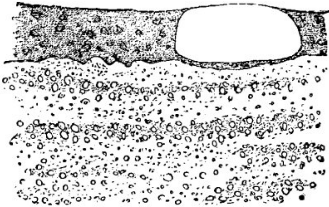
SECTION AT JOINVILLE.
