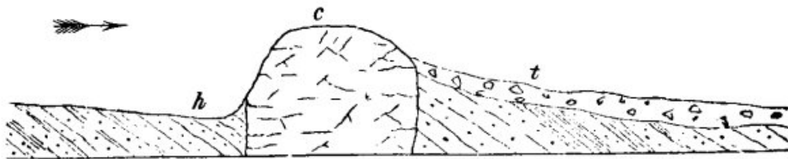
CRAG AND TAIL.-- c , crag; t , till.
