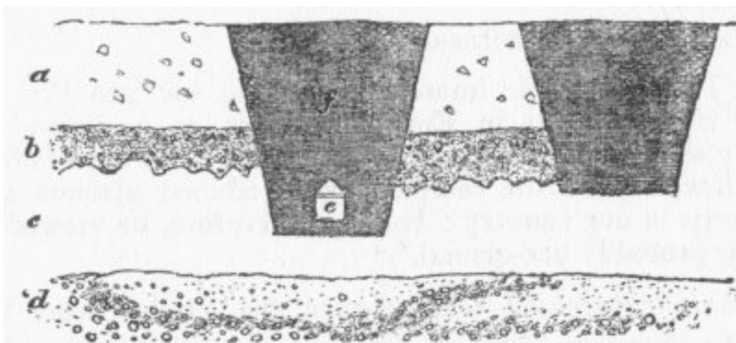
SECTION AT ST. ACHEUL.
