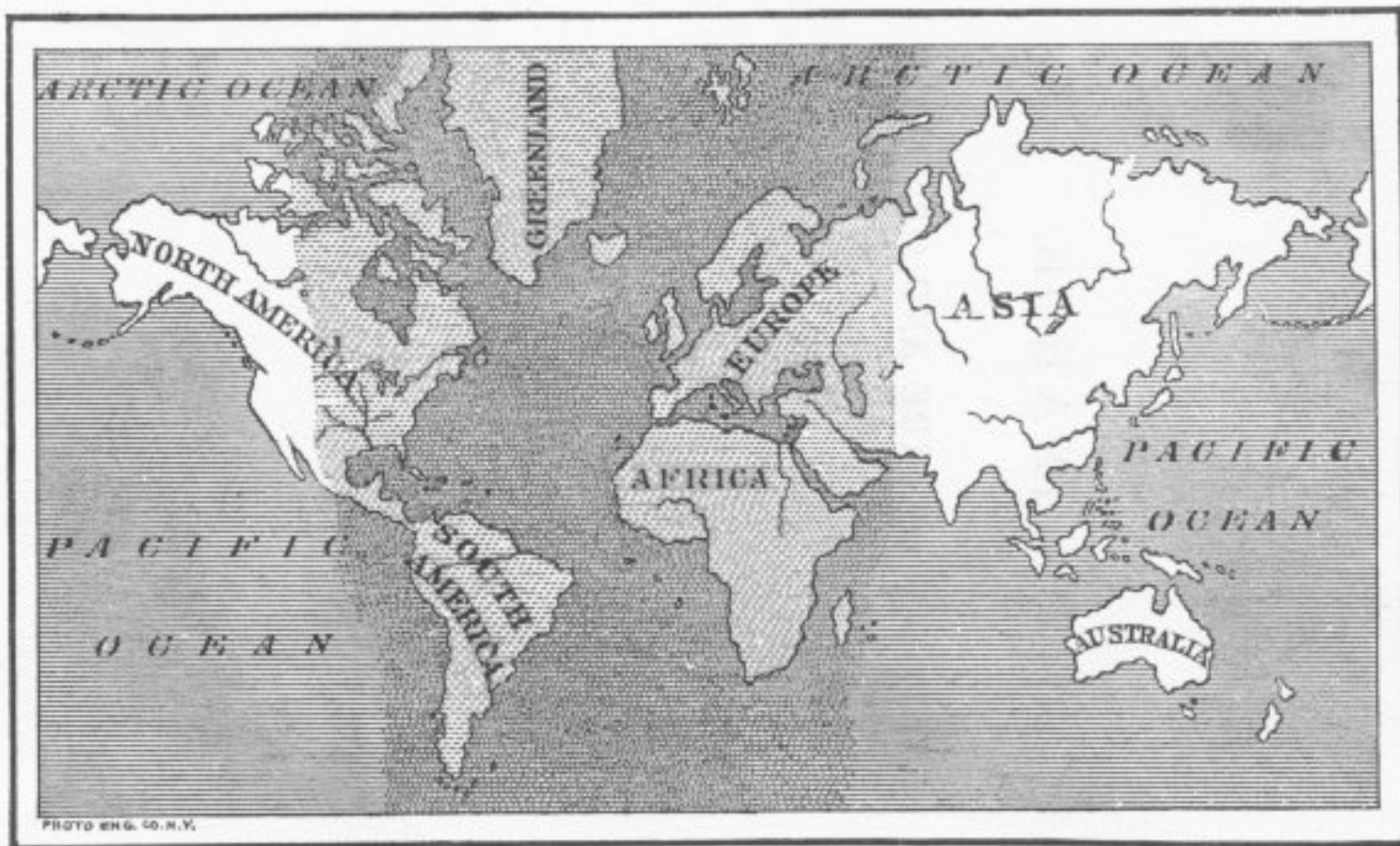
THE GEOGRAPHICAL DISTRIBUTION OF THE DRIFT.
