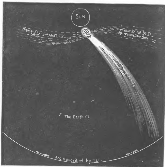
THE COMET SWEEPING PAST THE EARTH.
