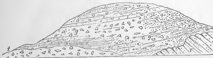
TILL OVERLAID WITH BOWLDER-CLAY, RIVER STINCHAR. r, Rock; t, Till; g, Boulder-Clay; x, Fine Gravel, etc.
