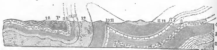
SECTION ON THE SCHUYLKILL, PENNSYLVANIA.
