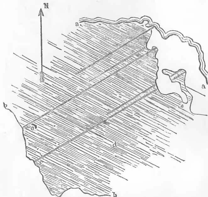
SKETCH OF GLACIER-FURROWS AND SCRATCHES AT STONY POINT, LAKE ERIE, MICHIGAN.
