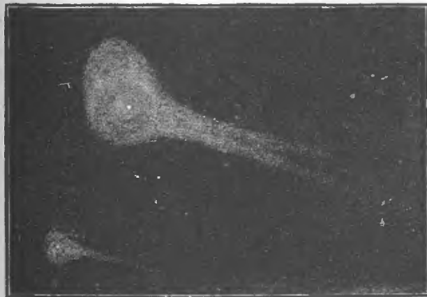
BIELA'S COMET, SPLIT IN TWO. (From Guillemin's "The Heavens," page 247.)
