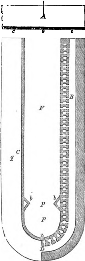
A is the boundary wall at the aphesis, 77 feet deep, B C the sides, and D the semicircular end, of the same depth as A; F F the area, including the σφενδομή ; b b pieces of masonry jutting out into the area; e e the entrances; from o to P is the
