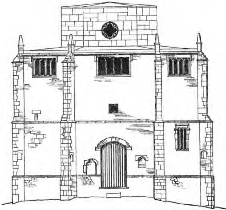
WEST ELEVATION
