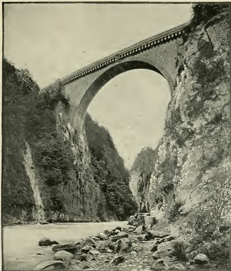
THE BRIDGE BUILT BY NAPOLEON III AT ST. SAUVEUR.
