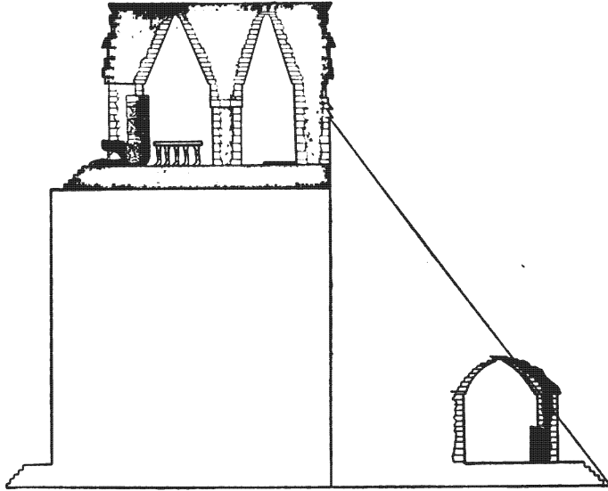
VERTICAL SECTION.
