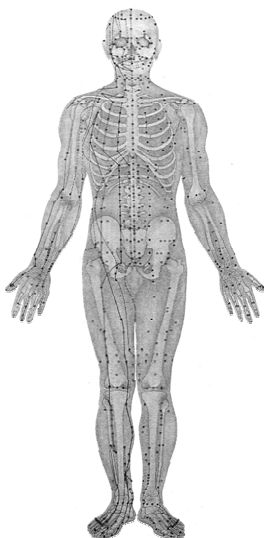
Figure 14. The number (361) of yods needed to construct the triakis tetrahedron from tetractyses is the number of acupoints in the human body.
