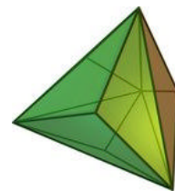
Figure 14. The number (361) of yods needed to construct the triakis tetrahedron from tetractyses is the number of acupoints in the human body.
