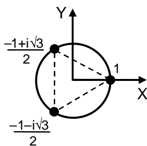
Figure 24. The three cubic roots of unity.
