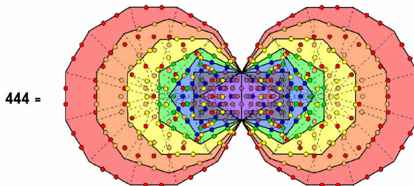
Figure 23. The inner Tree of Life has 444 hexagonal yods.
