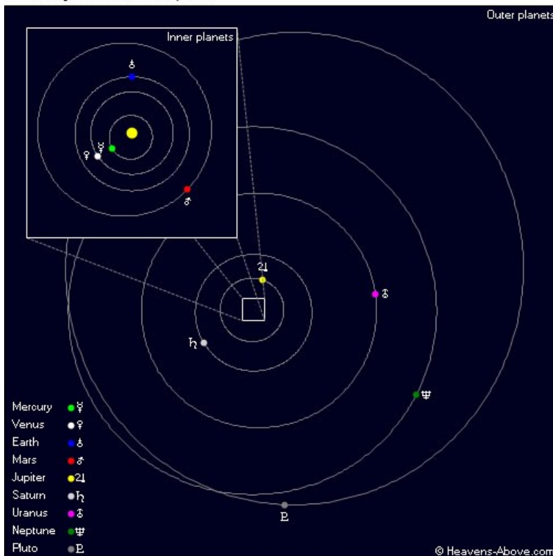
Solar-System on Dec. 21, 2012
