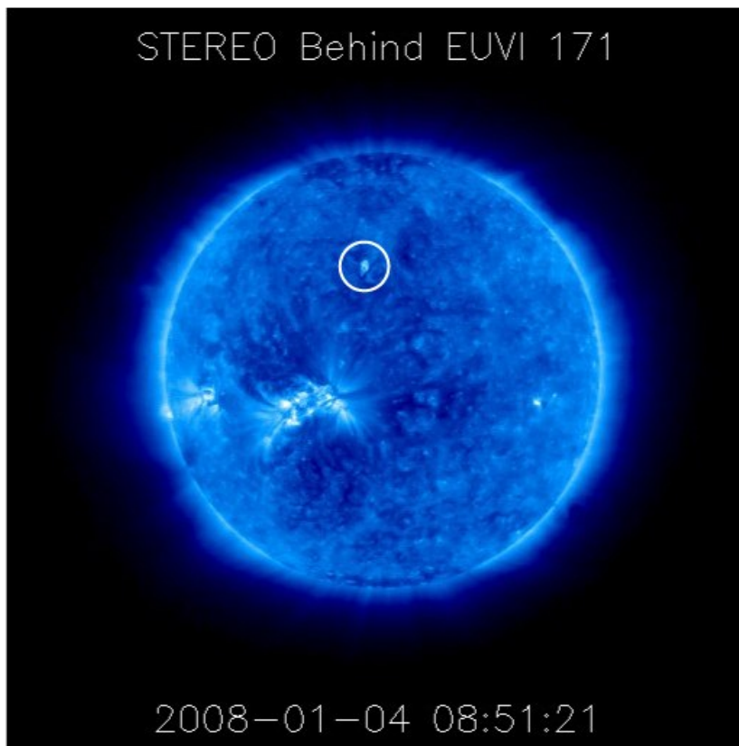
The first official active region of solar cycle 24 as it appeared to the STEREO Behind spacecraft observing in ultraviolet light on January 4, 2008. STEREO Behind was trailing Earth in its orbit by more than 20 degrees at the time.
