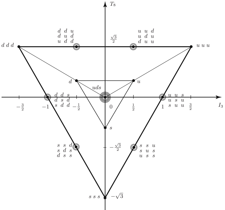
Figure 7. 3 \otimes 3 \otimes 3 = 10 \oplus 8 \oplus 8 \oplus 1 .
