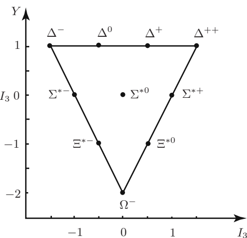
Figure 10b. The baryon resonances.
