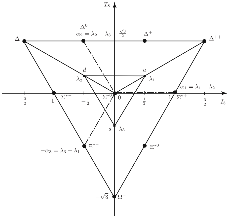
Figure 5. The representation \mathbf{10} .
