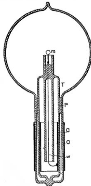
TYPE OF BULB WITHOUT LEADING-IN WIRE.
