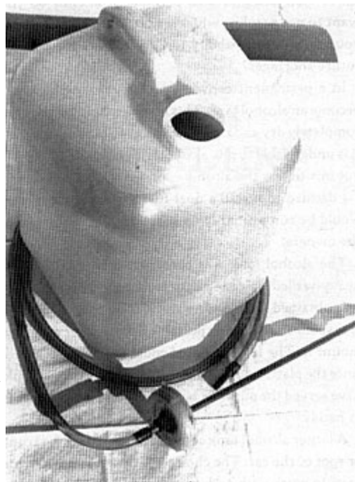
Figure 4-1 - This is my homemade 5-gallon fuel tank and pickup tube. Everything shown was scrounged up at no cost whatsoever.
