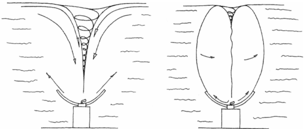
Figure 4.1: [A] Schauberg's oxygenator [B] Since the induced motion mainly is a rotating one, a water body is created, with little contact with the surrounding water.
