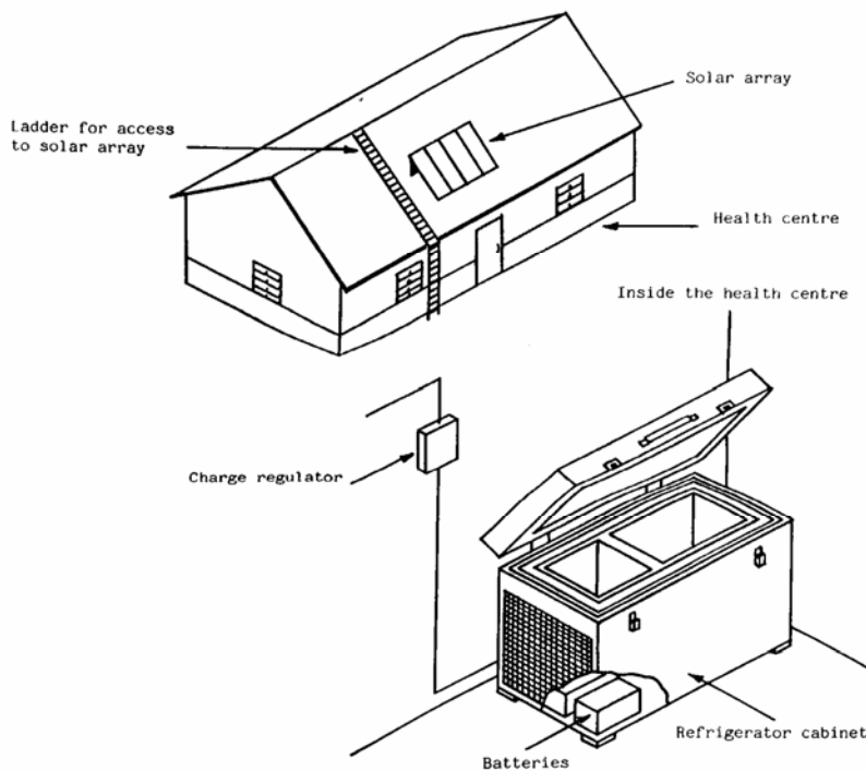
Figure 1: A typical refrigerator layout
