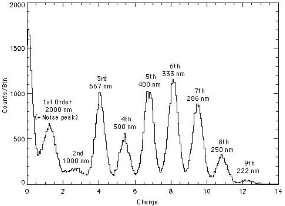
Figure 13.27 Tantalum STJ response to input from a grating monochromator, with intensity plotted against collected charge. (Courtesy of ESA.)
