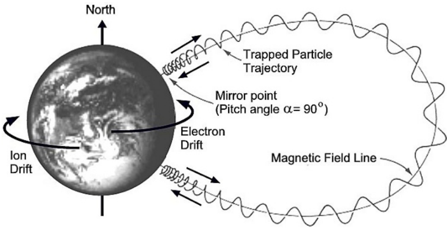
Figure 4.5 The motion of charged particles on dipole-like field lines in near-Earth space. Particles gyrate around the field, bounce between low-altitude mirror points in both the north and south hemispheres and drift around the Earth. Ions and electrons drift in opposite directions, thus contributing to a ‘ring current’ around the Earth. Particles are trapped on such field lines, so these are the main processes leading to the formation of the Van Allen radiation belts. (After Spjeldvik and Rothwell, 1985.)
