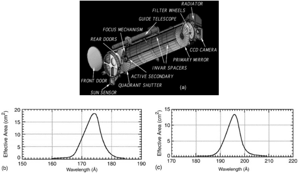
Figure 13.44 (a) TRACE EUV telescope. Three of the four mirror quadrants have Mo 2 C/Si coatings. (b) Multilayer response at 17.3 nm and (c) at 19.5 nm. The third quadrant response is centred at 28.4 nm. (Courtesy of Lockheed and NASA.)
