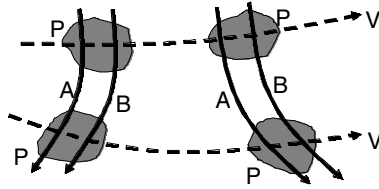
Figure 4.8 The concept of frozen-in magnetic flux 2. In a highly conducting plasma, in which the scale lengths are large, the magnetic field is frozen in. As a result, two volumes of plasma, P_1 and P_2 , which are originally linked by fields lines A and B, will remain connected by field lines A and B, whatever the individual motions V_1 and V_2 of the individual volumes.
