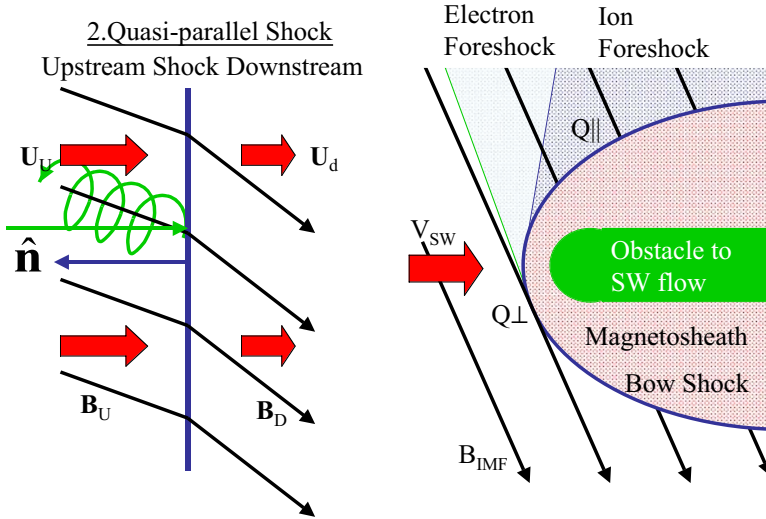
Figure 4.11 Field and flow structure in the vicinity of a quasi-parallel shock, at which the upstream magnetic field, B_U , is close to being parallel to the shock normal \mathbf{n} . The flow speed decreases through the shock such that the density and magnetic field strength increase in the downstream region. A fraction of particles (e.g. as indicated by the grey trajectory) may be reflected at the shock and in this magnetic field configuration may rapidly escape along the magnetic field back into the upstream region. (b) Large-scale structure upstream of an obstacle to the solar wind flow. Shocked plasma between the bow shock and the obstacle itself forms the magnetosheath region. The bow shock itself generally has both quasi-perpendicular and quasi-parallel regions. Upstream of the quasi-parallel shock, particles escaping back upstream form the extended foreshock regions. Since electrons move much faster than ions, they are able to reach regions further upstream than the latter.
