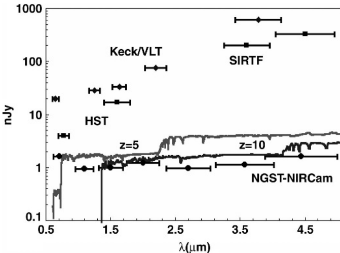
Figure 13.39 Sensitivity (nJy) of a NGST Near IR Camera design (Rieke et al. , 2001) for z \leq 10 galaxies ( 5\sigma , 50,000 \text{ s} ). (Courtesy of M. Rieke.)
