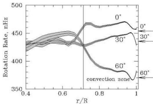
Figure 6.5 This shows the inferred rotation rate as a function of depth and latitude within the Sun. This has been determined at three different latitudes (equator, 30^\circ and 60^\circ ). Courtesy of SOHO/MDI consortium. SOHO is a project of international cooperation between ESA and NASA.
