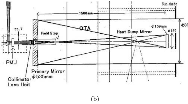
Figure 13.40 Solar-B 0.5 m telescope mounting (a) truss structure, primary and secondary mirrors, heat dump mirror and thermal radiation paths. (b) Solar radiation paths, operation of heat dump mirror and connection to focal plane instruments through collimator lens and polarisation modulator unit (PMU). (c) Collimator lens unit. (Courtesy of ISAS.)
