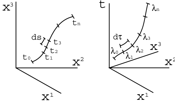
Figure 10.8 Left : The motion of a particle in a three-dimensional space. The position of the particle is specified by the time parameter t . The separation of two spatial points along the particle trajectory is ds . Right : The motion of a particle in a four-dimensional space–time as a consequence of events. The events are specified by a parameter \lambda . The interval between two events is d\tau .
