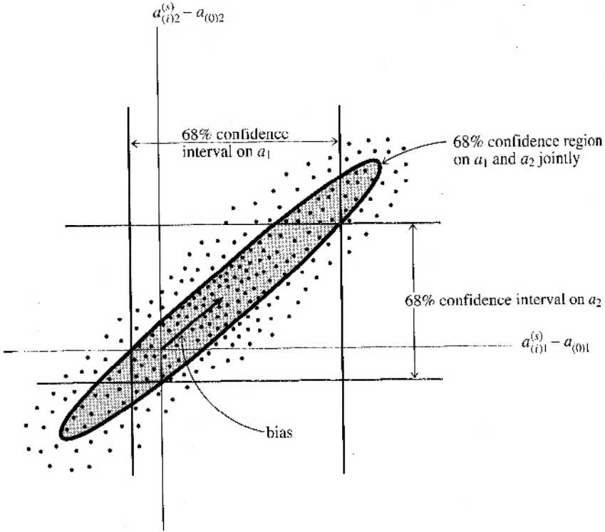
Figure 12.8 Plot of all the best fits in the two dimensions of the parameter space with contour encompassing 68% of them. (From Numerical Recipes , Press et al. , 1996.)
