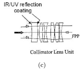
Figure 13.40 Solar-B 0.5 m telescope mounting (a) truss structure, primary and secondary mirrors, heat dump mirror and thermal radiation paths. (b) Solar radiation paths, operation of heat dump mirror and connection to focal plane instruments through collimator lens and polarisation modulator unit (PMU). (c) Collimator lens unit. (Courtesy of ISAS.)
