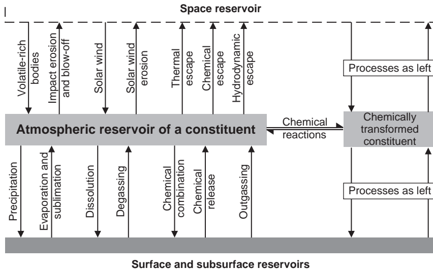
Figure 9.10 The reservoirs of some atmospheric constituent, and the various types of process by which it can be transferred from one reservoir to another.
