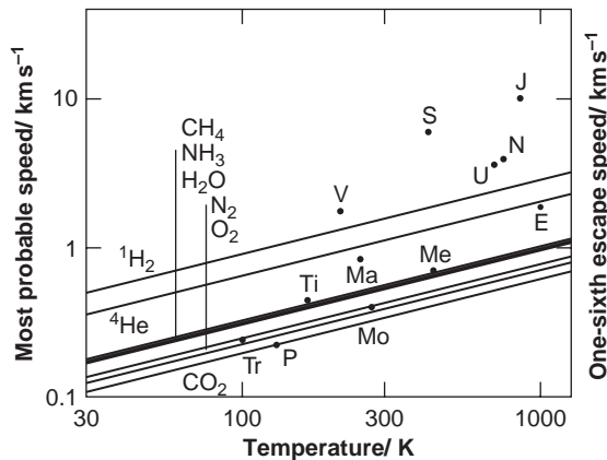
Figure 9.12 The most probable speed v_{mps} versus temperature T for some major atmospheric gases. Planetary bodies are at the temperatures at the base of their exospheres.
