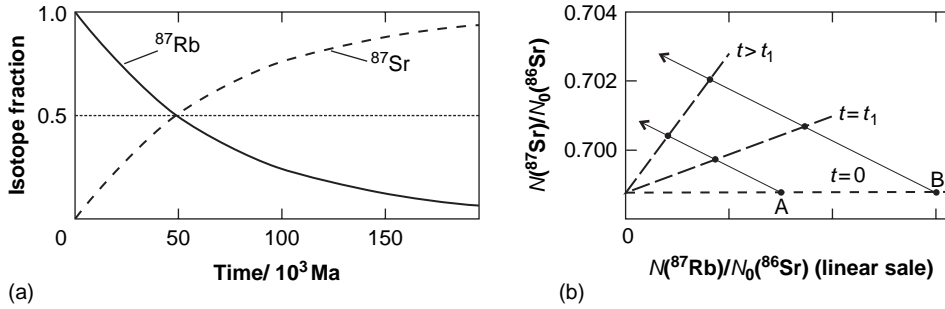
Figure 3.15 (a) The principle of radiometric dating using the decay of 87 Rb into 87 Sr. (b) The Rb–Sr isochron plot for two minerals, A and B. The dashed lines are isochrons at three different times.
