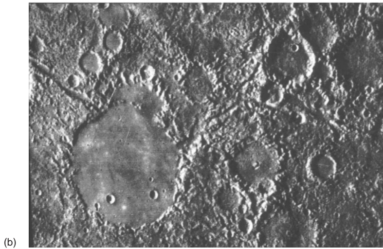
Figure 7.5 (a) The Caloris Basin on Mercury. Note the ejecta, the multiple rings, the infill, the smooth plains. The inner ring is about 1300 km in diameter. (NASA/NSSDC AoM F21) (b) Hilly terrain diametrically opposite the Caloris Basin. The largest crater, Petrarch, is about 150 km across. (NASA/NSSDC FDS27370)
