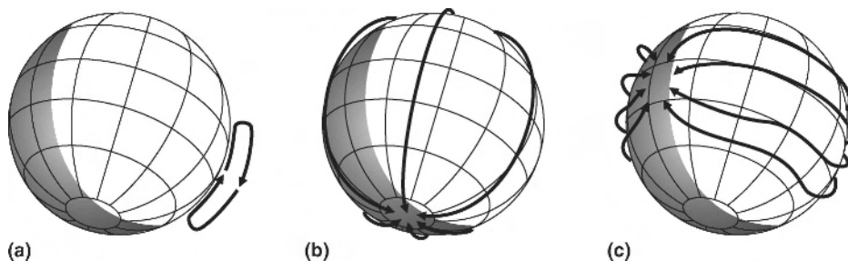
Figure 10.9 Atmospheric circulation in the lower atmosphere of Mars. (a) Hadley cell. (b) Condensation flow. (c) Thermal flow. (Adapted by permission from Figure 5 (p97) of The New Solar System , J K Beatty and A Chaikin (eds.), Sky Publishing, 1990)
