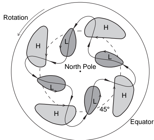
Figure 9.15 Mid-latitude atmospheric waves.
