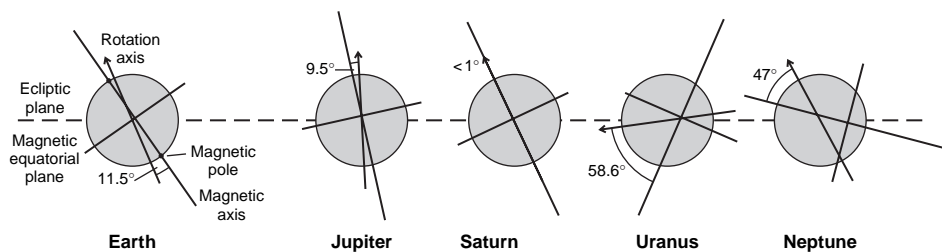
Figure 4.6 The magnetic axes of the five planetary bodies that have large dipole moments.
