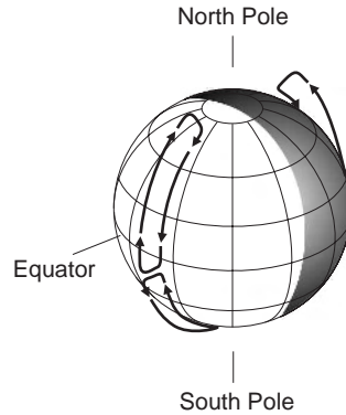
Figure 9.13 A single Hadley cell per hemisphere on a slowly rotating terrestrial planet with a small axial inclination.
