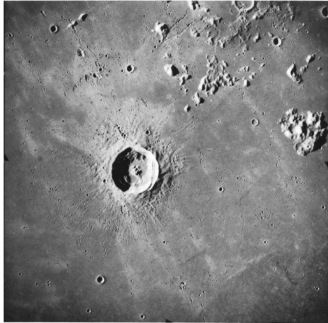
Figure 6.11 Rays, secondary craters, and an ejecta blanket from the lunar crater Euler (27 km in diameter). (NASA/NSSDC AS17-2923)
