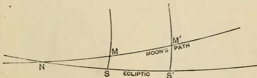
FIG. 26.—The ecliptic and the moon's path.
