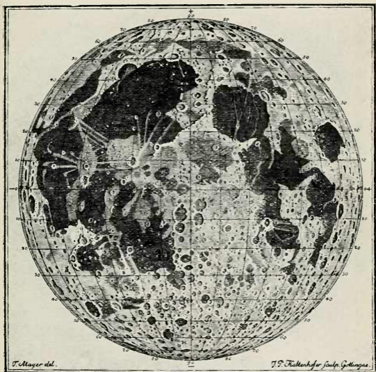
FIG. 79.—Tobias Mayer's map of the moon.
