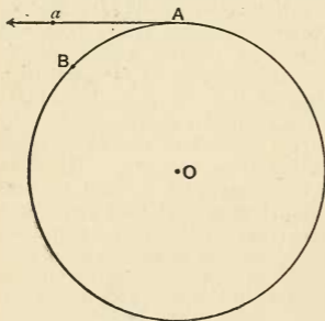
FIG. 70.—Motion in a circle.
