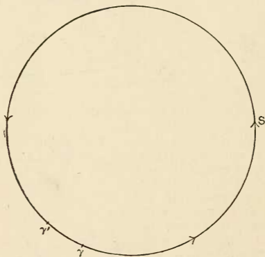
FIG. 24.—The precession of the equinoxes.
