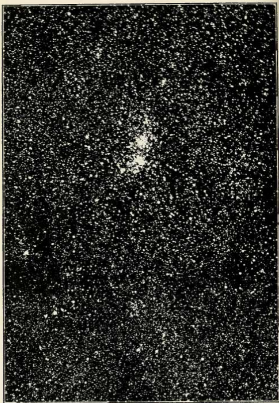
FIG. 104.—The Milky Way near the cluster in Perseus. From a photograph by Professor Barnard. [To face p. 405.]
