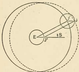
FIG. 45.—The epicycle of Jupiter.
