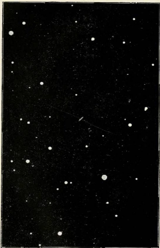
FIG. 88. Photographic trail of a minor planet.
