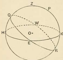
FIG. 15.—The equator, the horizon, and the meridian.
