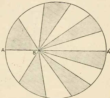
FIG. 60.—Kepler's second law.
