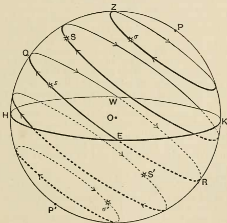
FIG. 3.—The circles of the celestial sphere.
