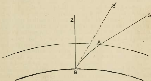
FIG. 32.—Refraction by the atmosphere.
