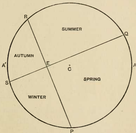
FIG. 18.—The position of the sun's apogee.
