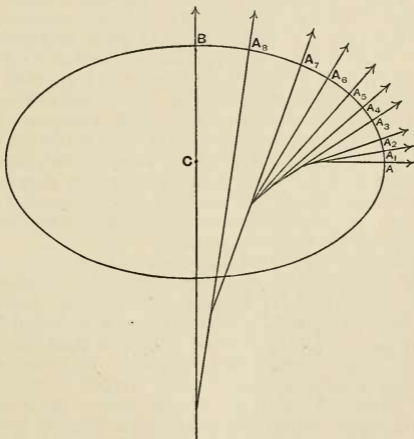
FIG. 78.—The varying curvature of the earth.
