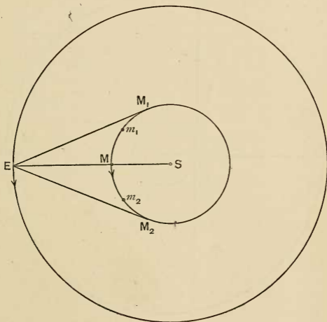
FIG. 47.—The stationary points of Mercury.
