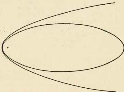
FIG. 73.—An elongated ellipse and a parabola.
