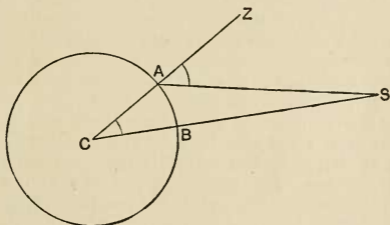
FIG. 16.—The measurement of the earth.
