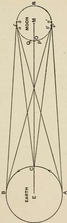
FIG. 58.—The daily libration of the moon.
