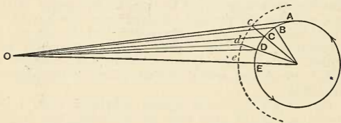
FIG. 56.—Galilei's proof that sun-spots are not planets.
