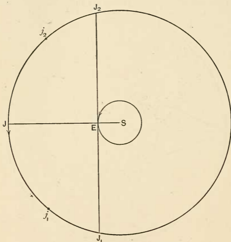
FIG. 48.—The stationary points of Jupiter.
