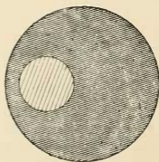
FIG. 29.—Total eclipse of the moon.
