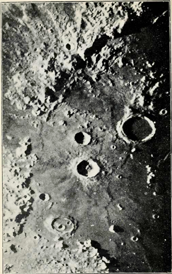
FIG. 94.—The Apennines and adjoining regions of the moon. From a photograph taken at the Paris Observatory. [To face p. 383.]
