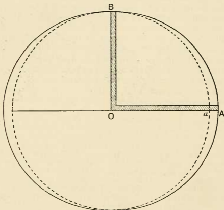
FIG. 72.—The spheroidal form of the earth.
