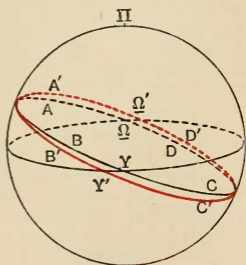
FIG. 23.—The precession of the equinoxes.
