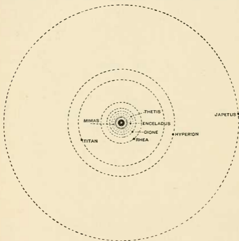
FIG. 91.—Saturn and its system.
