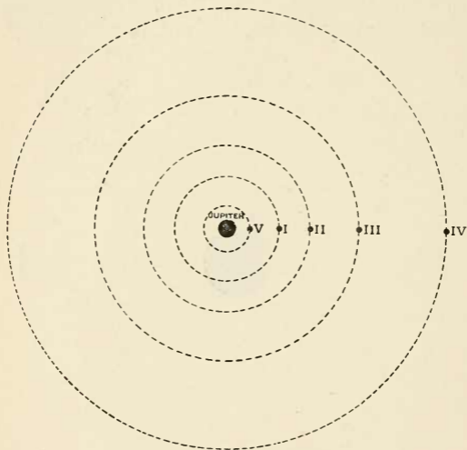
FIG. 93.—Jupiter and its satellites.
