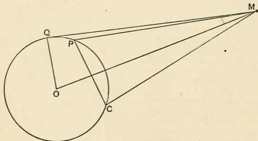
FIG. 69.—The parallax of a planet.
