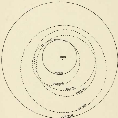
FIG. 89.—Paths of minor planets.
