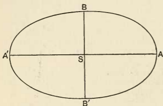
FIG. 76.—The aberrational ellipse.
