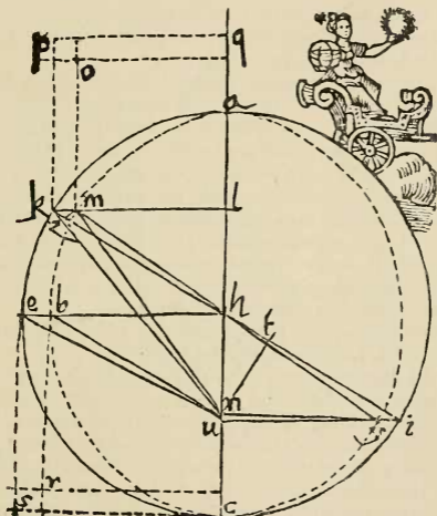
FIG. 61.—Diagram used by Kepler to establish his laws of planetary motion. From the Commentaries on Mars .
