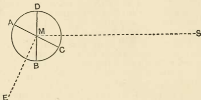
FIG. 8.—The phases of the moon.
