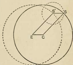
FIG. 19.—The epicycle and the deferent.
