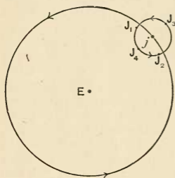
FIG. 34.—Jupiter's epicycle and deferent.
