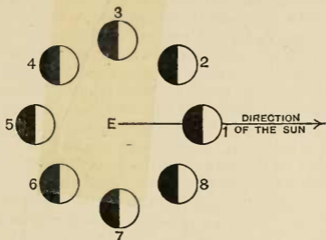
FIG. 10.—The phases of the moon.
