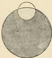
FIG. 28.—Partial eclipse of the moon.
