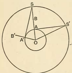
Fig. 39.—The daily rotation of the earth.
