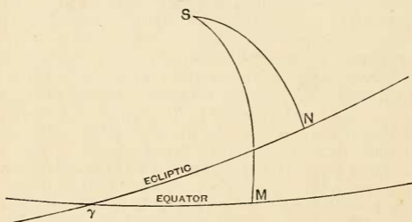
FIG. 14.—The equator and the ecliptic.
