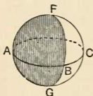
FIG. 9.—The phases of the moon.
