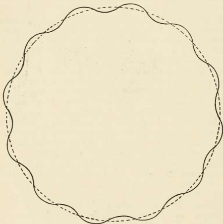
FIG. 77.—Precession and nutation.
