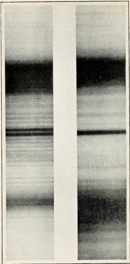
FIG. 103.—The spectrum of \beta Aurigae, shewing the K line single and double. From a photograph taken at Harvard. [To face p. 403.]
