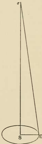
FIG. 86.—The parallax of 61 Cygni.
