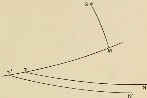
FIG. 22.—The movement of the equator.
