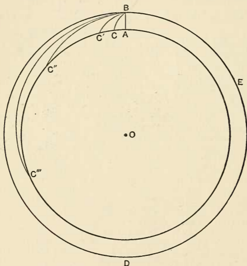
FIG. 71.—The moon as a projectile.
