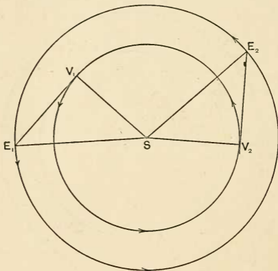
FIG. 44.—The synodic and sidereal periods of Venus.
