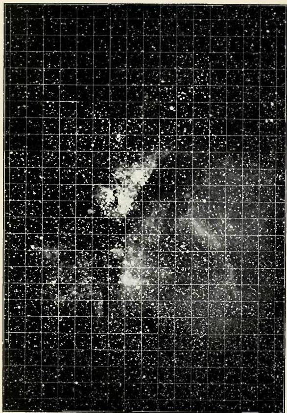
FIG. 100.—The nebula about \eta Argus. From a photograph by Dr. Gill L. [To face p. 397.]
