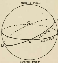
FIG. 4.—The equator and the ecliptic.
