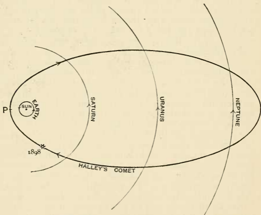
FIG. 80.—The path of Halley's comet.
