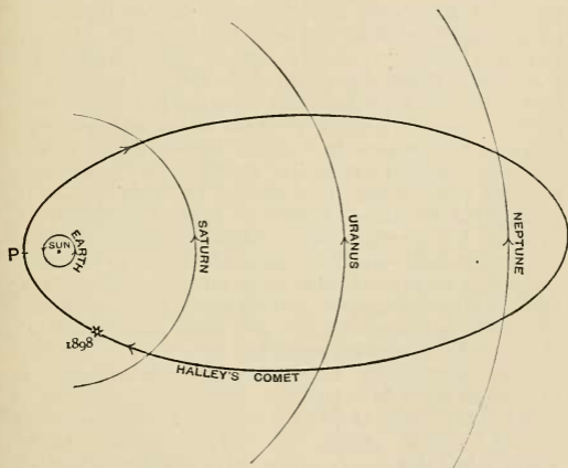
FIG. 87.—The path of Halley's comet.
