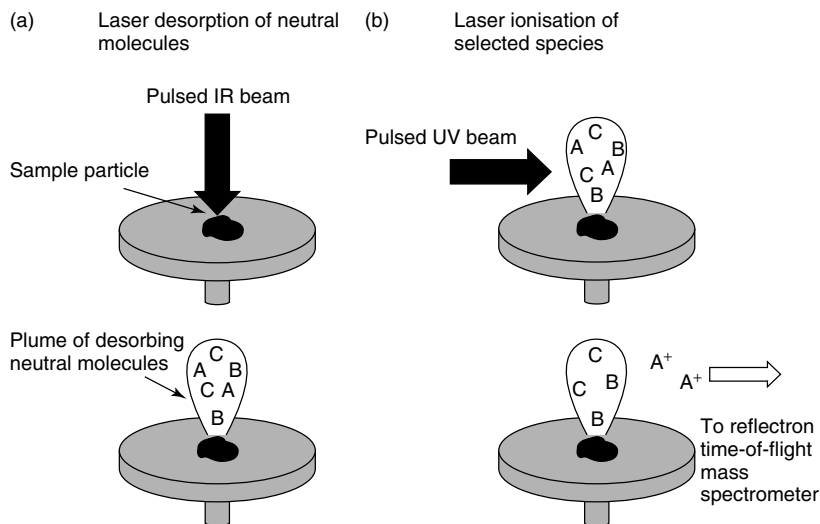
Figure 6.5 The \mu\text{L}^2\text{MS} technique consists of (a) laser desorption followed by (b) laser ionisation to selectively produce ions, that are then extracted into a time-of-flight mass spectrometer for mass analysis. (Reproduced by permission of R.N. Zare, Stanford University)
