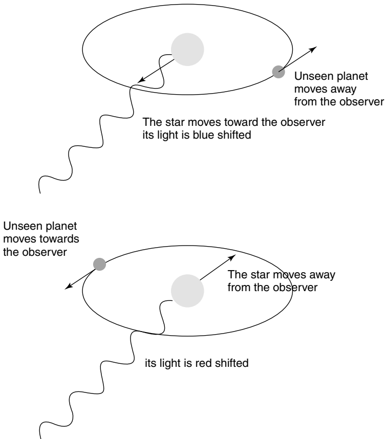
Figure 7.8 Doppler shift due to the presence of a planet around a star
