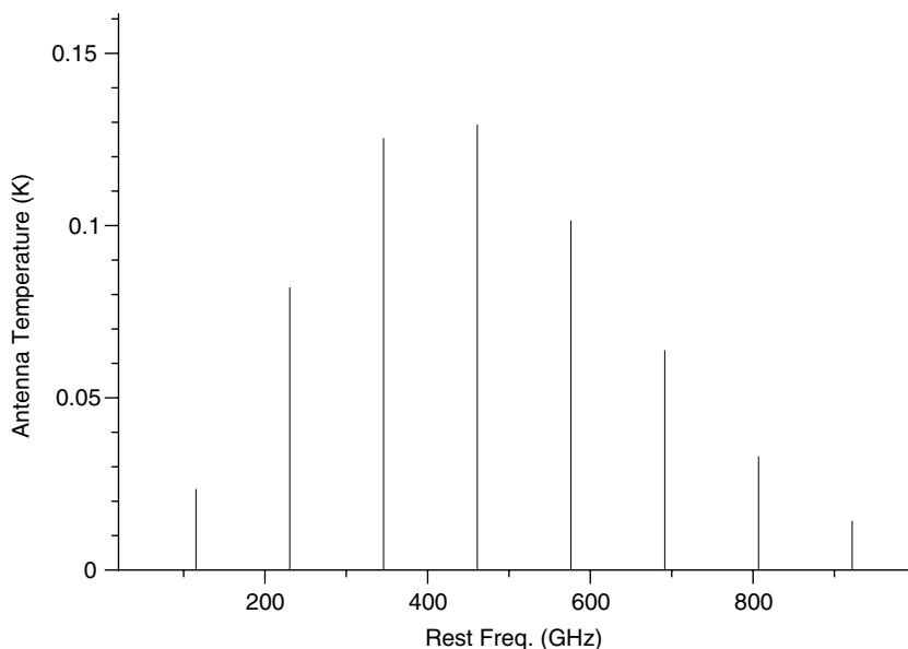
Figure 3.7 Simulated spectrum of CO with a rotational temperature of 40 K. Reproduced by with permission of Albert Nummelin, Chalmers University of Technology
