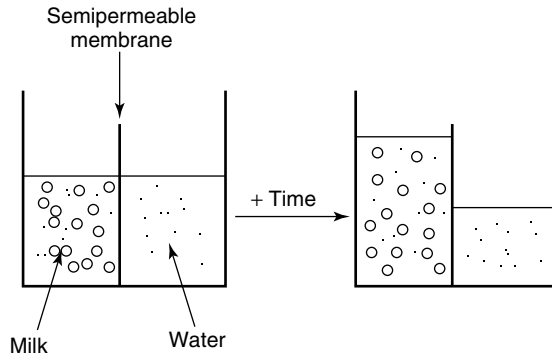
Figure 9.9 Osmotic pressure
