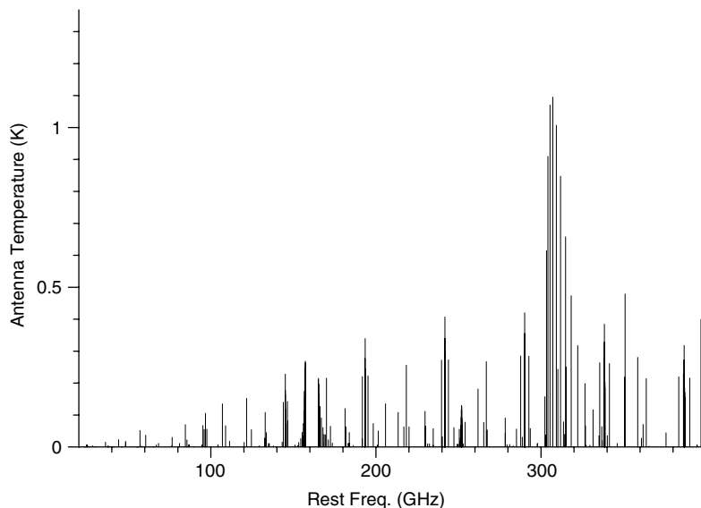
Figure 3.9 Simulated spectrum of \text{CH}_3\text{OH} at 40 K. Reproduced by permission of Albert Nummelin, Chalmers University of Technology
