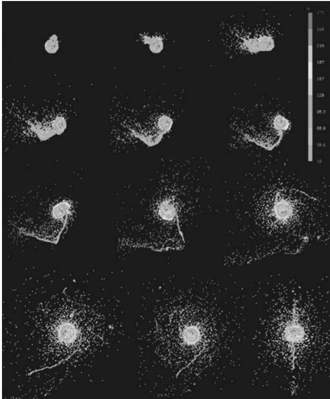
Figure 7.4 Modelling of the Moon-capture event. (Reproduced by permission of Southwest Research Institute)
