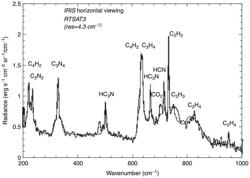
Figure 10.3 Voyager I IRIS spectrum of the northern limb of Titan. (Reproduced by permission of Voyager Missions, JPL NASA)
