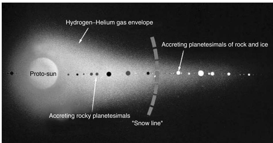
Figure 6.19 Snow line
