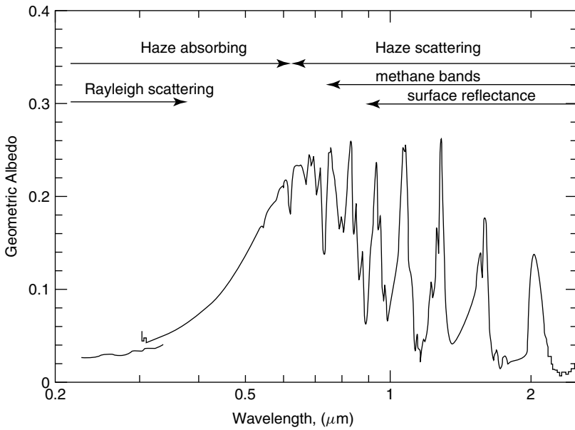
Figure 10.4 Reflection spectrum. (Reproduced by permission of Dr. Chris McKay, NASA Ames)
