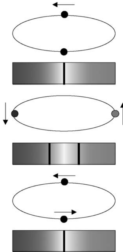
Figure 4.13 Doppler effect for a binary star pair
