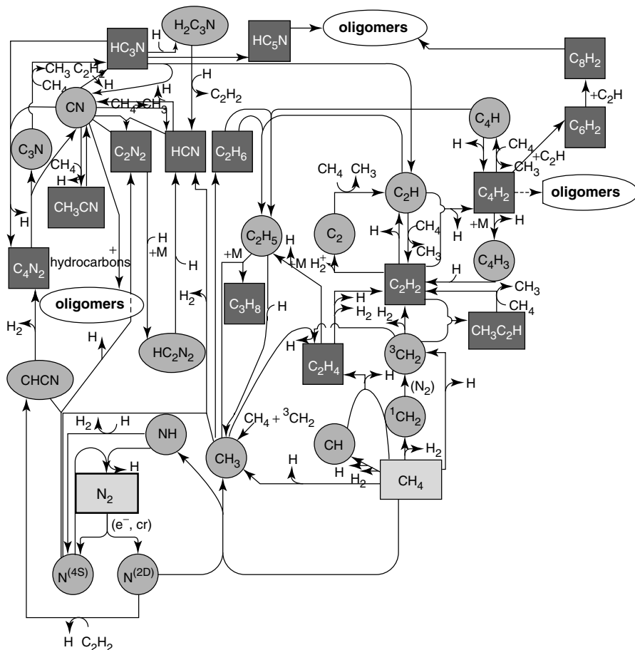
Figure 10.8 Chemical network based on \text{CH}_4 and \text{N}_2 . (Adapted with permission from Yung et al. 1984)
