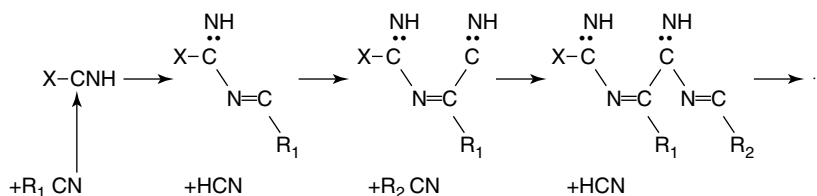
Figure 10.10 Nitrile polymerisation
