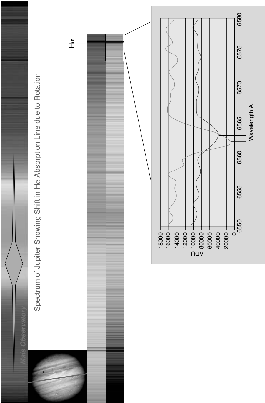
Figure 3.2 The reflection spectrum of Jupiter. (Reproduced by courtesy of Dale Mais, Mais Observatory)
