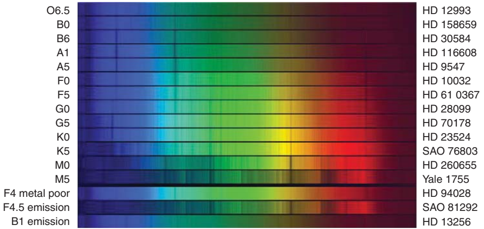
Figure 4.2 Spectra from different stellar classes OBAFGKM. (Reproduced by permission of KPNO 0.9-m Telescope, Aura, NOAO, NSF)
