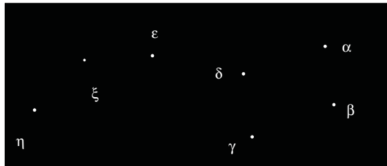
Figure 2.10 Labelling of the stars in Ursa Major
