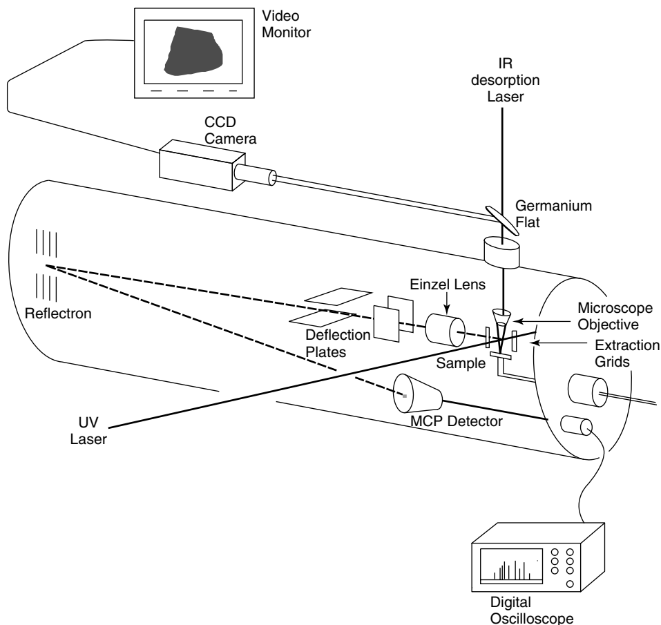
Figure 6.6 A time-of-flight mass spectrometer. The arrival time of the ions is proportional to the mass. (Reproduced by permission of R. N. Zare, Stanford University)
