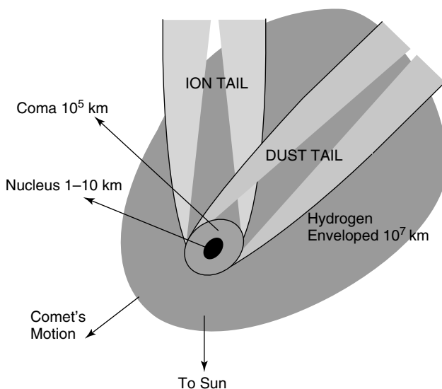
Figure 6.16 Structure of the comet showing the nucleus, the coma and two tails – an ion tail and a dust tail
