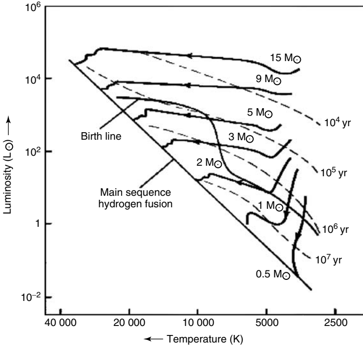
Figure 4.4 Birth lines for stars descending onto the main sequence, where M_{\odot} denotes solar mass
