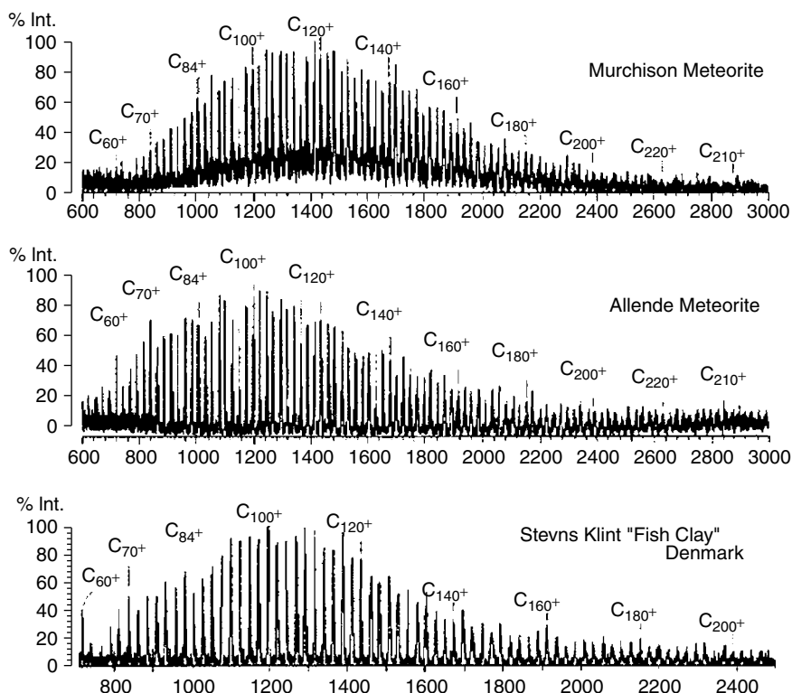
Figure 6.9 Laser desorption mass spectra of extracts of the Murchison and Allende carbonaceous chondrites and an extraction from the K/T boundary. (Adapted from Becker L, Poreda R. J. and Bunch T. E., 2000 by permission of the Proceedings of the National Academy of Sciences 97 : 2979)
