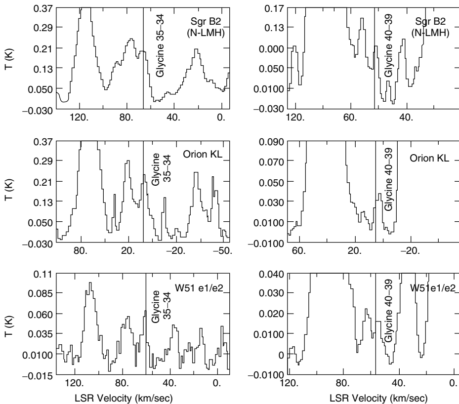
Figure 5.24 Glycine spectra (at 1 MHz resolution) observed at 206,468 MHz (line 21) in (a) Sgr B2(N-LMH), (b) Orion KL, and (c) W51 e1/e2 and at 240,899 MHz (line 26) in (d) Sgr B2(N-LMH), (e) Orion KL, and (f) W51 e1/e2. The abscissae give the rest frequencies based on the assumed LSR velocities: 64.0, 8.0, and 60.0 km s -1 for Sgr B2(N-LMH), Orion KL, and W51 e1/e2, respectively. The thick vertical lines mark the glycine lines at the frequencies corresponding to the measured velocities. The thin vertical lines denote the spectral features of other molecular species; question marks indicate uncertain identifications because of overly strong line intensities or inconsistent LSR velocities. (Reproduced from the Astrophysical Journal 593:848-867, 2003 by permission of the AAS)
