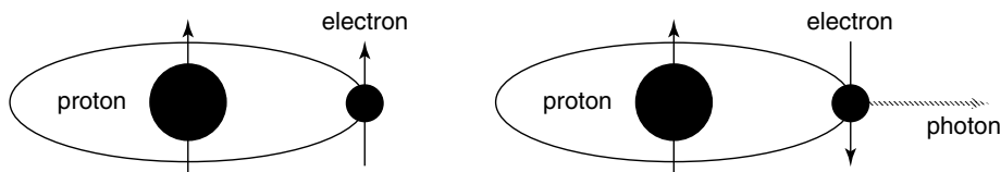
Figure 3.18 The 21-cm line in the H atom
