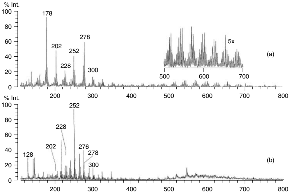
Figure 6.13 The \mu\text{L}^2\text{MS} spectrum of ALH84001: (a) from the carbonate granules; (b) from the bulk meteorite. (Reproduced from Becher 1999 with permission from Elsevier)
