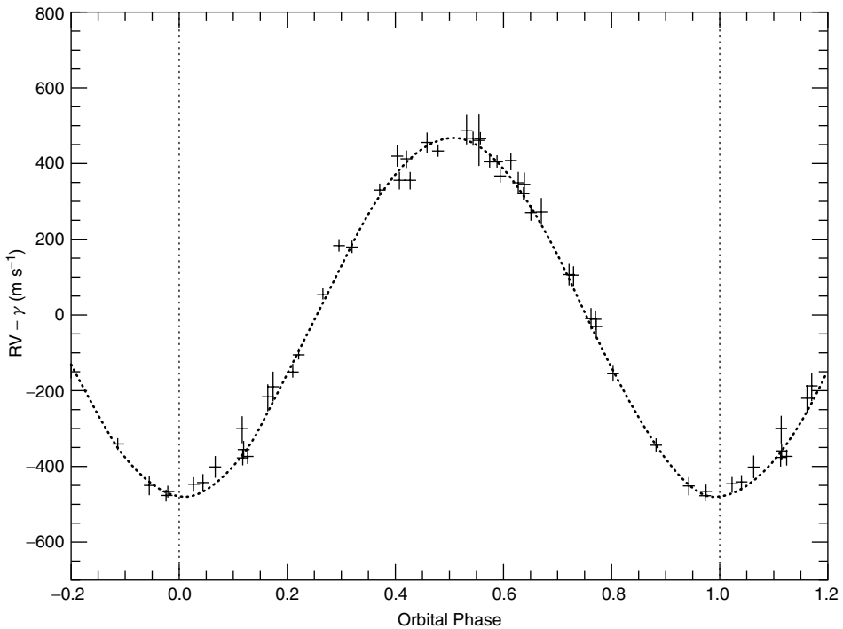
Figure 7.10 Radial velocity variations for \tau -Bootes. (Reproduced by permission of Sylvain Korzennik, Harvard-Smithsonian Center for Astrophysics)
