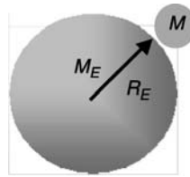
Figure 7.2 Gravitational weight
