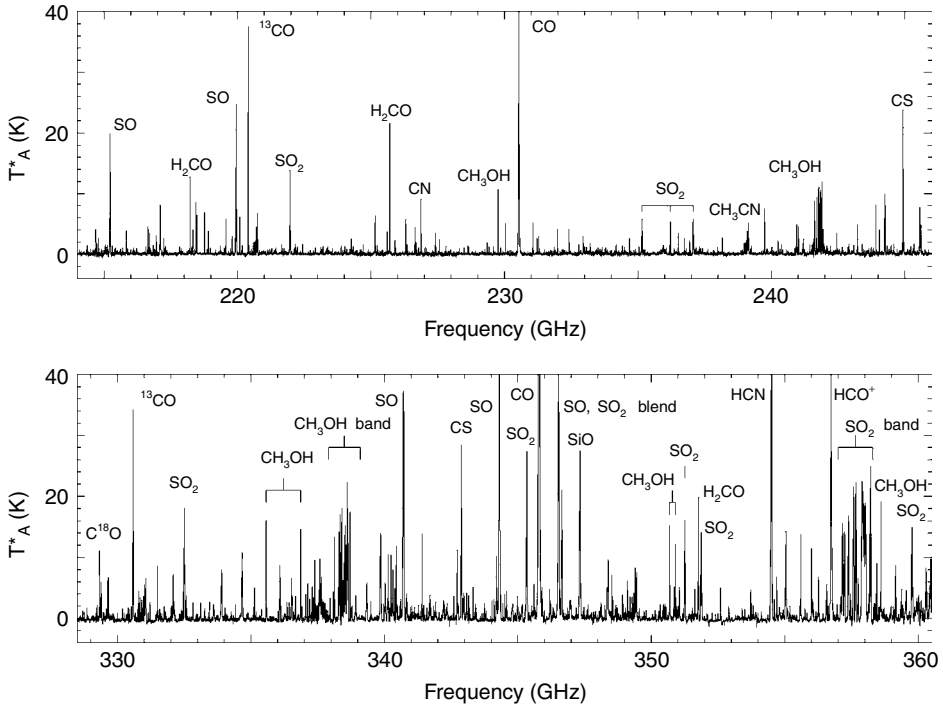
Figure 3.11 The microwave spectrum of the Orion nebula. Reproduced by permission of Geoffrey A. Blake, Owens Valley Radio Observatory
