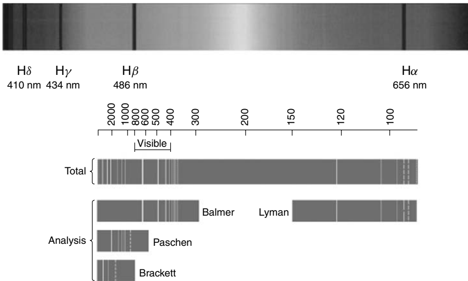
Figure 3.5 The hydrogen atom absorption spectrum and the named sequences. (Reproduced by permission of Pearson Publishing)
