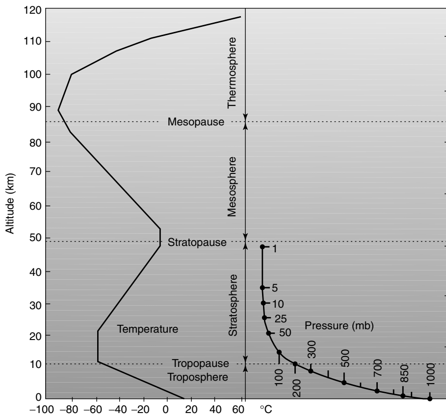
Figure 7.11 Temperature profile of the Earth's atmosphere. (Reproduced by permission of Oklahoma Geological Society)
