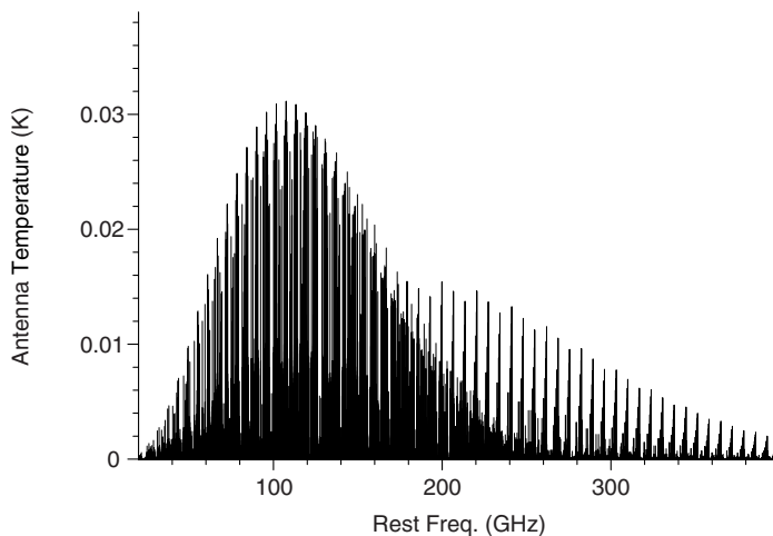
Figure 3.10 Simulated rotational spectrum of glycine at 40 K. Reproduced by permission of Albert Nummelin, Chalmers University of Technology
