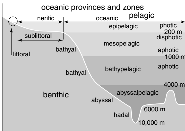
Figure 7.13 Oceanic zones
