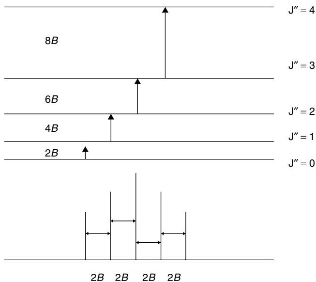
Figure 3.6 The energy-level diagram for a rotational spectrum
