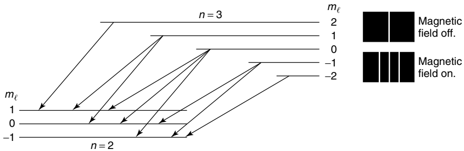
Figure 4.12 The origin of Zeeman splitting in the n = 2 - n = 3 transition in the H atomic spectrum
