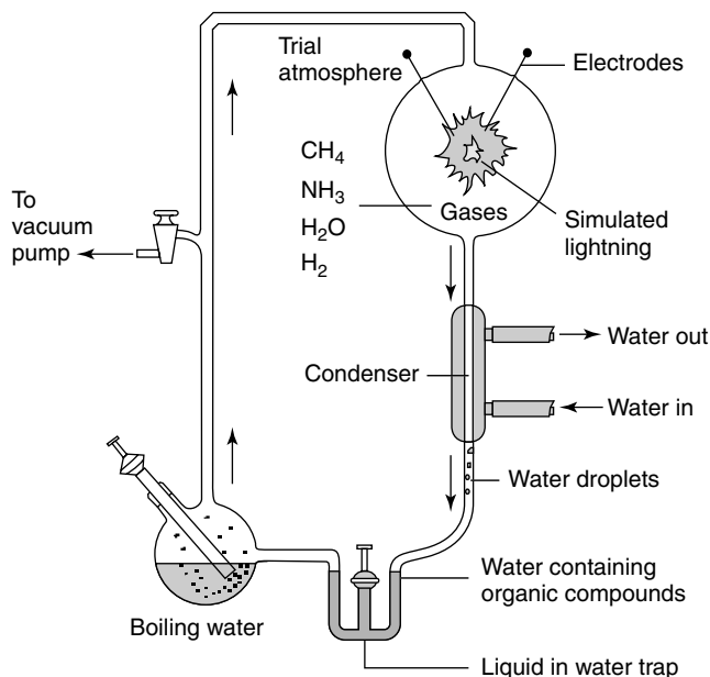
Figure 8.2 Urey–Miller experiments
